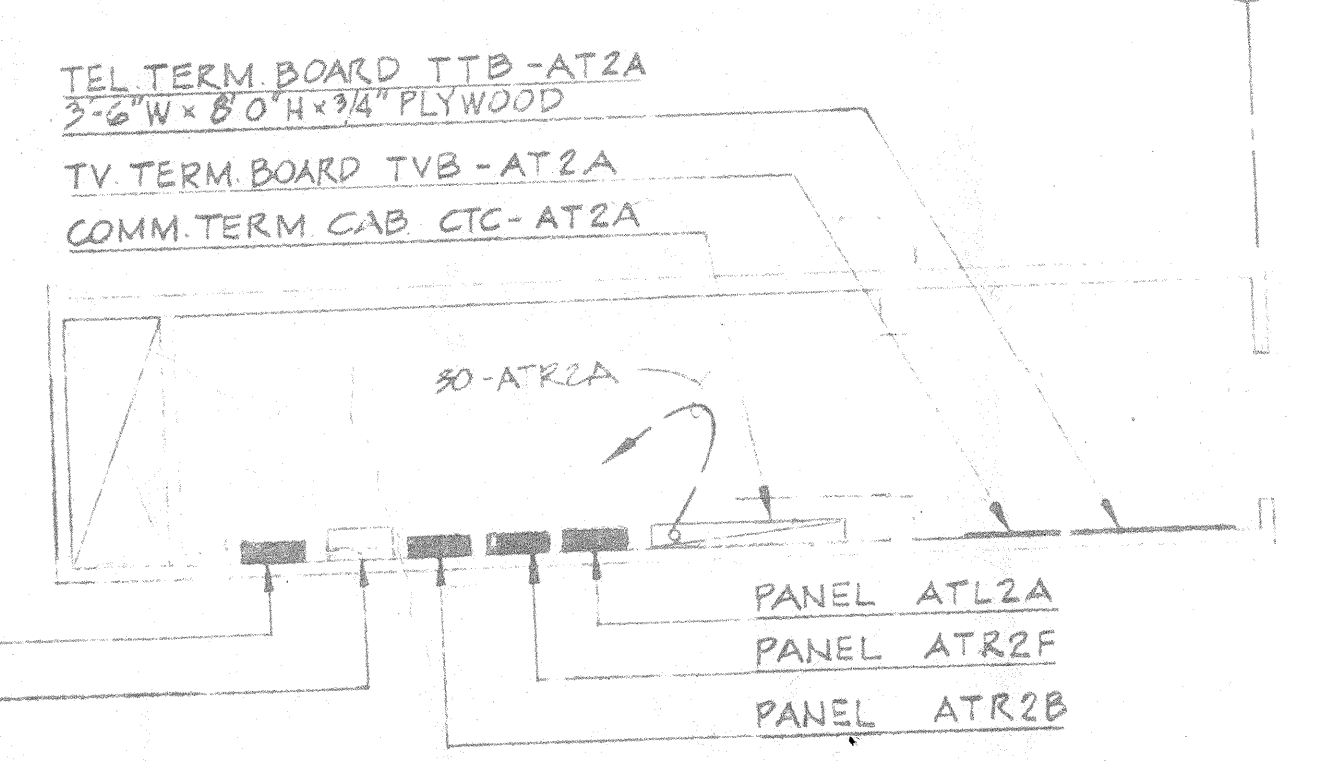
ELECTRIC CLOSET #475 SCALE 1/4"=1'-0"
