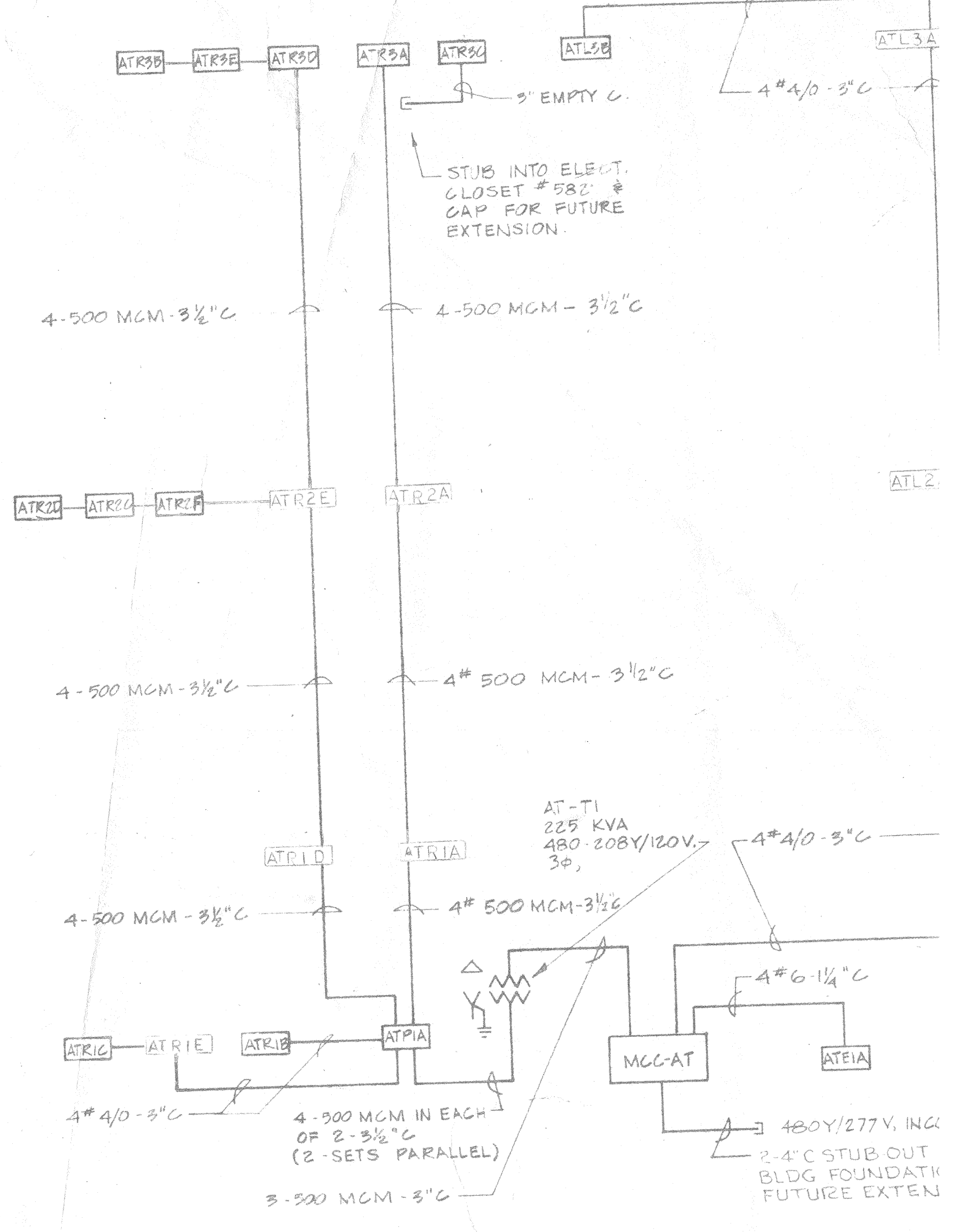
BUILDING "A" RISER DIAGRAM - (WEST PORTION)
