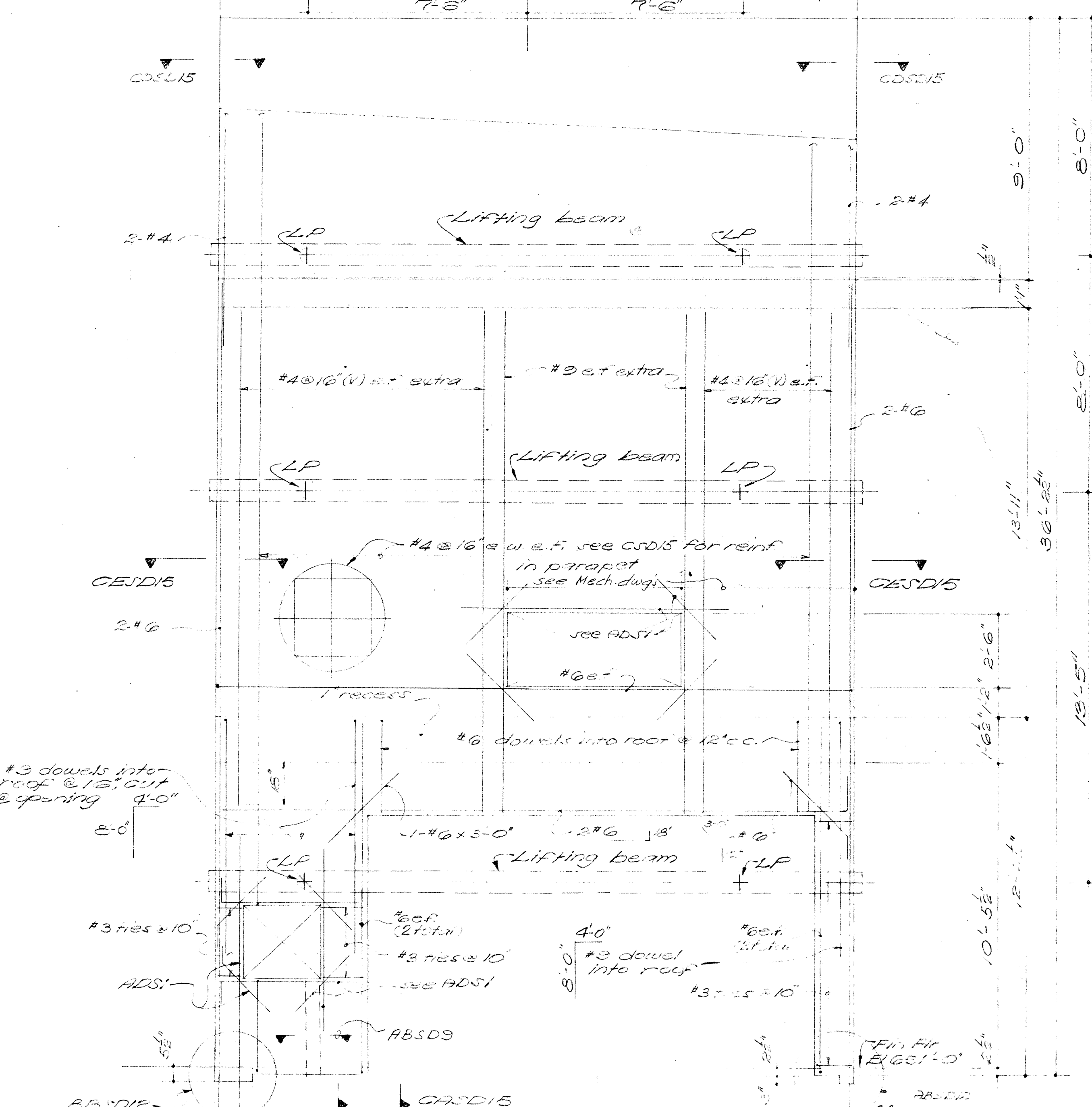
EASD9 10' WALL AT LINE A LOOKING WEST 3/4" = 1'-0"
