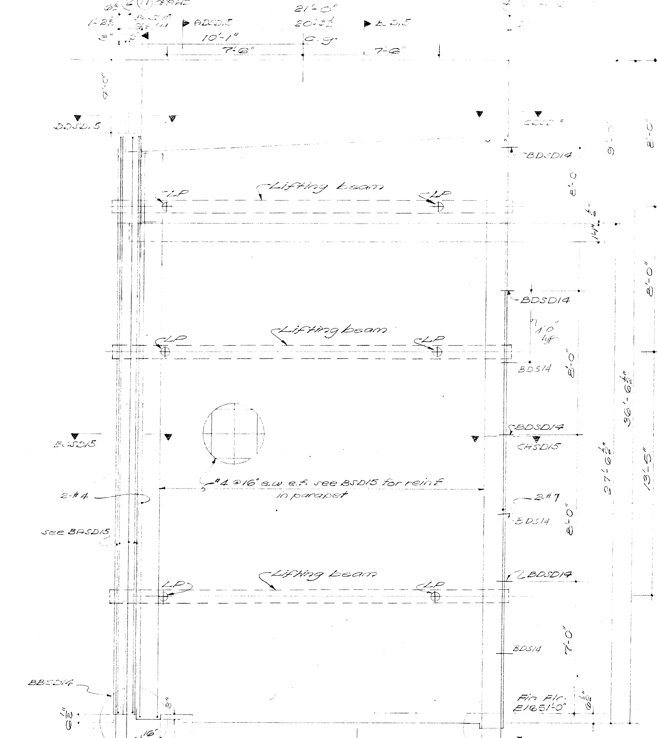
CSD9 10' WALL AT LINE B 3/4" = 1'-0"
