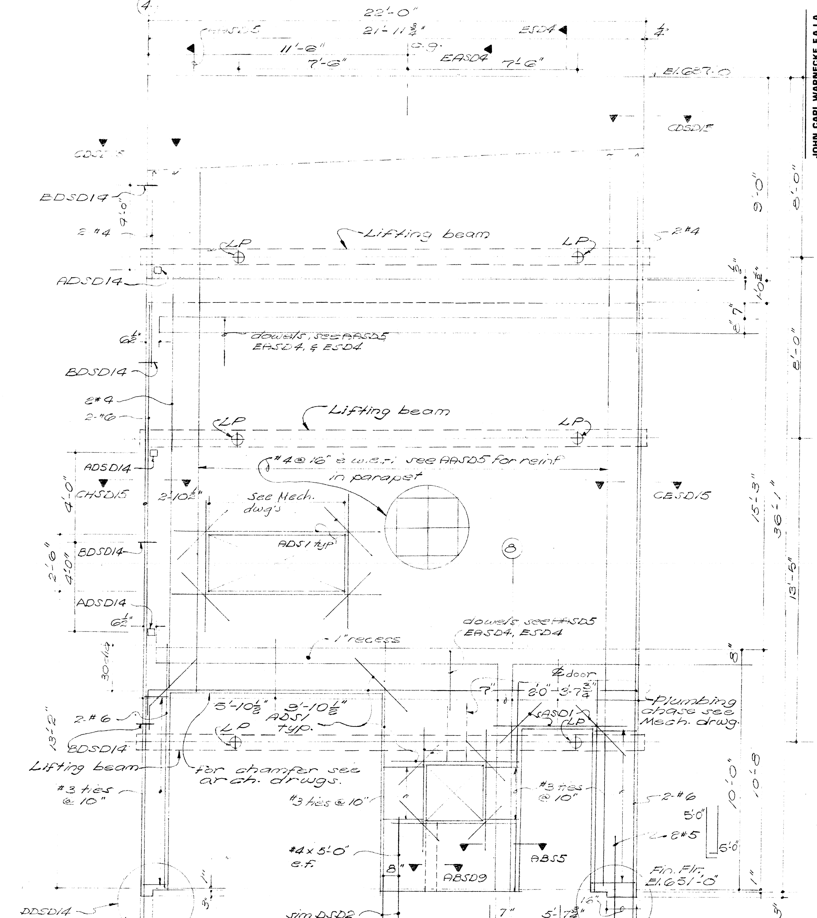
ASD9 10' WALL AT LINE C 3/4" = 1'-0"
