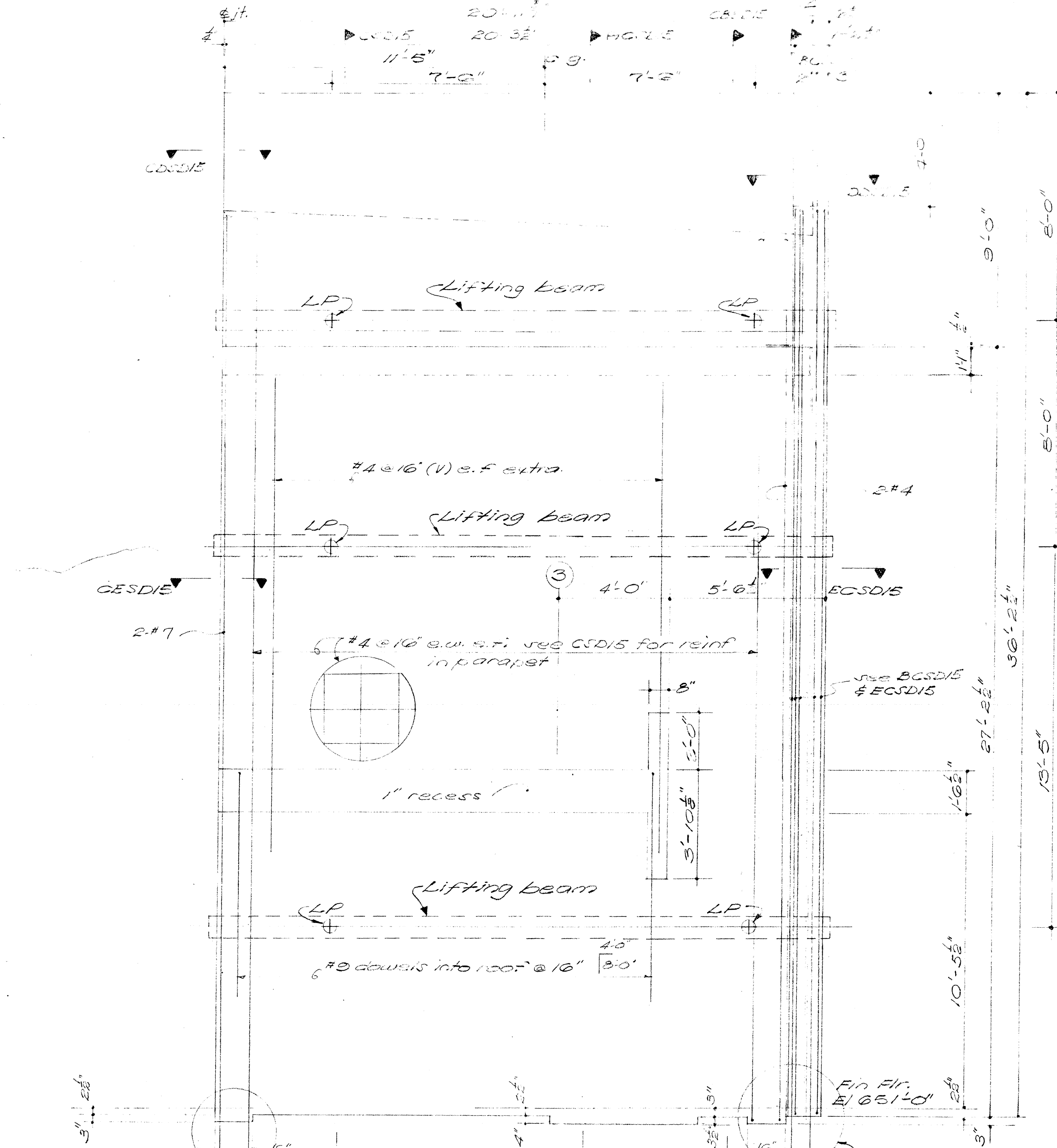
ESD9 10' WALL AT LINE A LOOKING WEST 3/4" = 1'-0"
