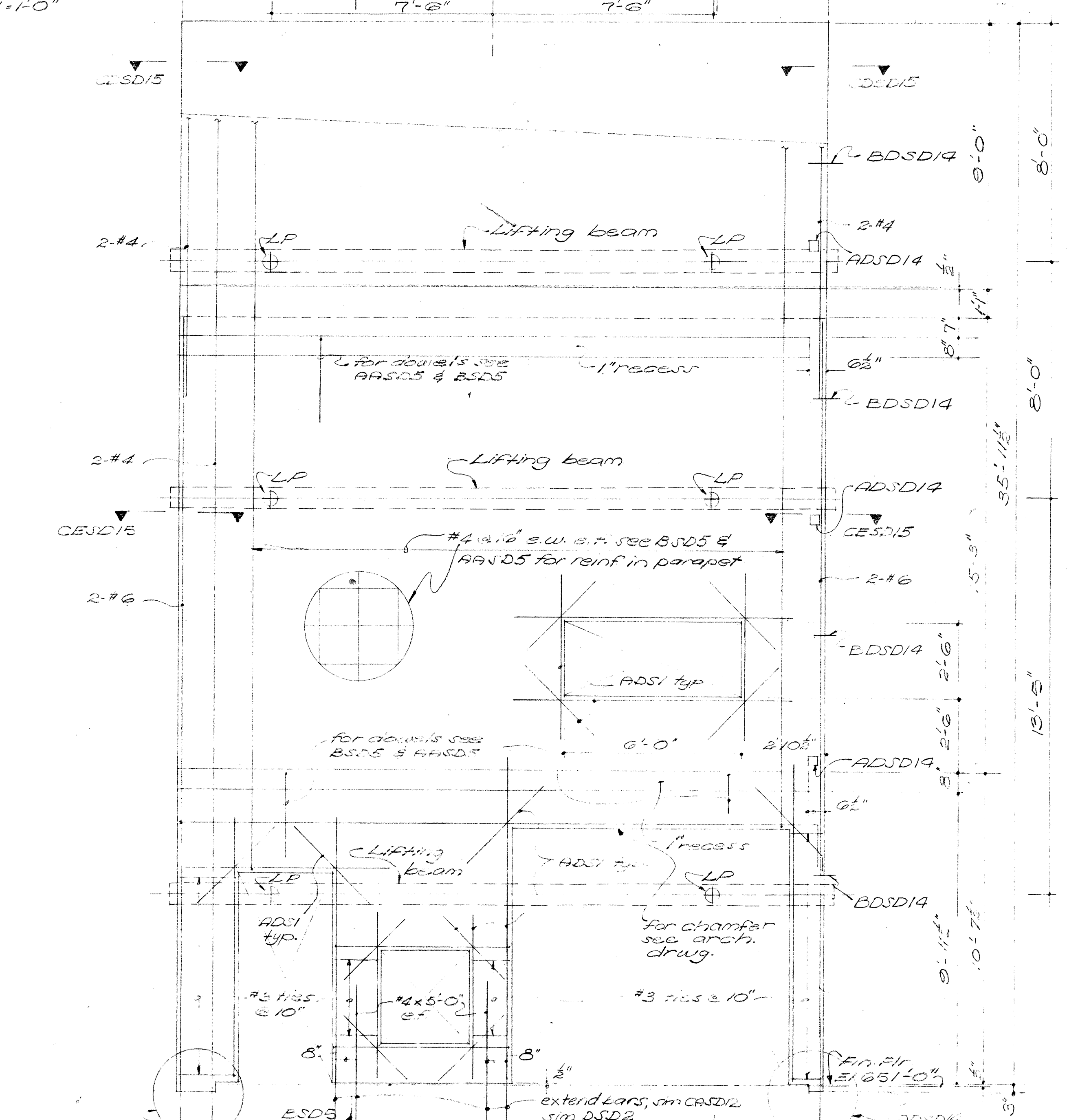
AASD9 10' WALL AT LINE C 3/4" = 1'-0"
