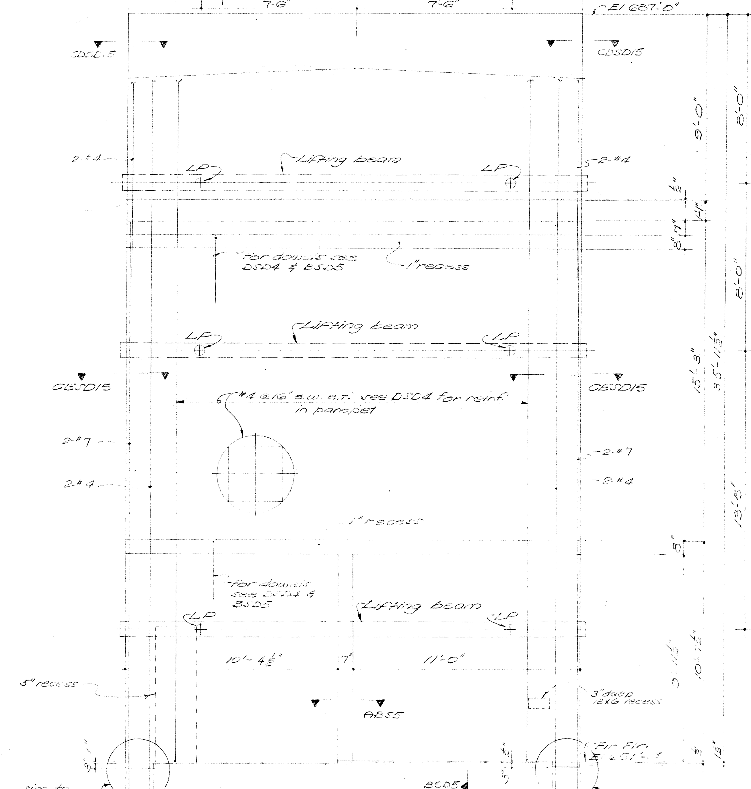
CASD9 10' WALL AT LINE B 3/4" = 1'-0"
