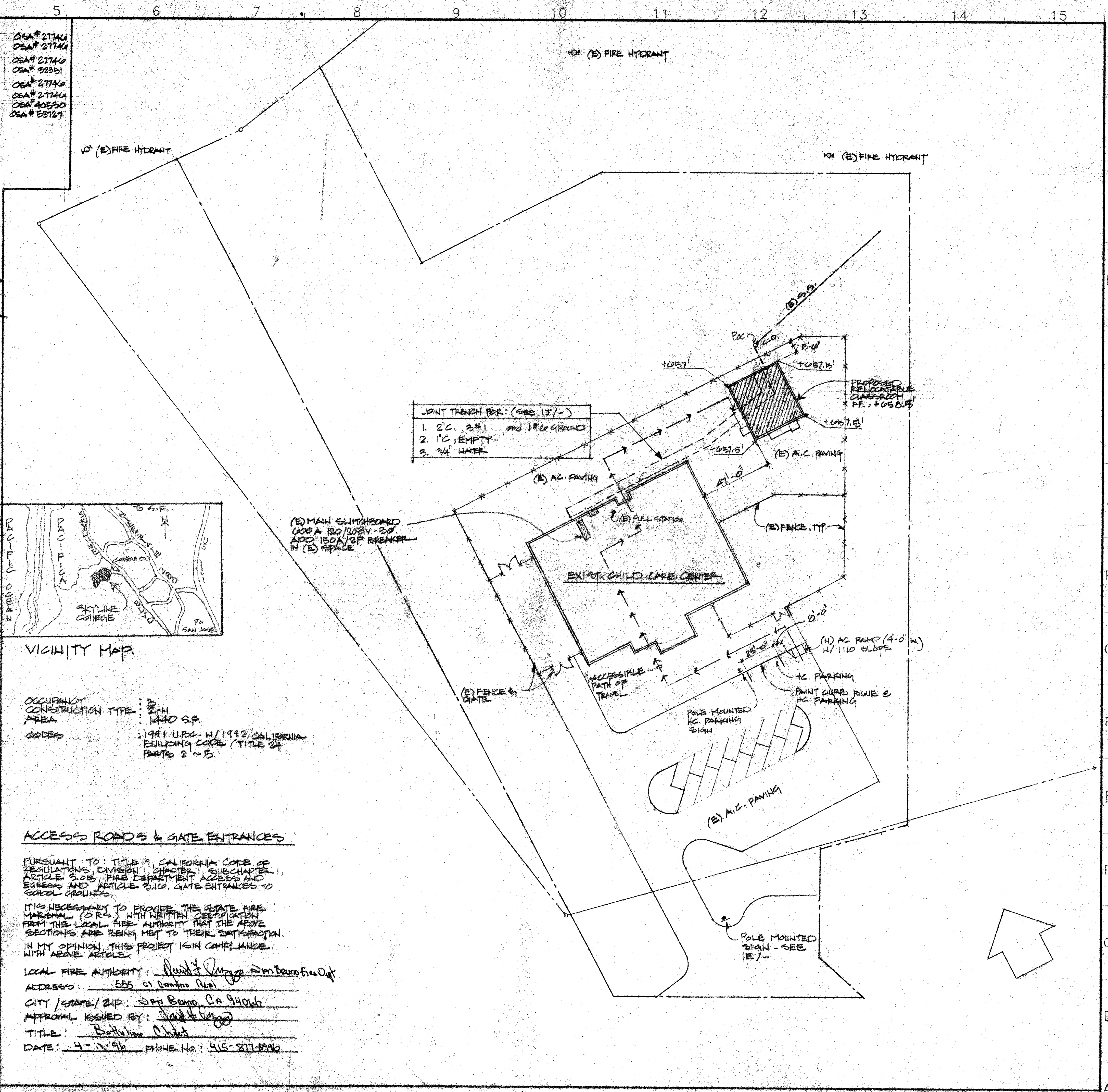
SITE PLAN 1/8" = 1'-0"
