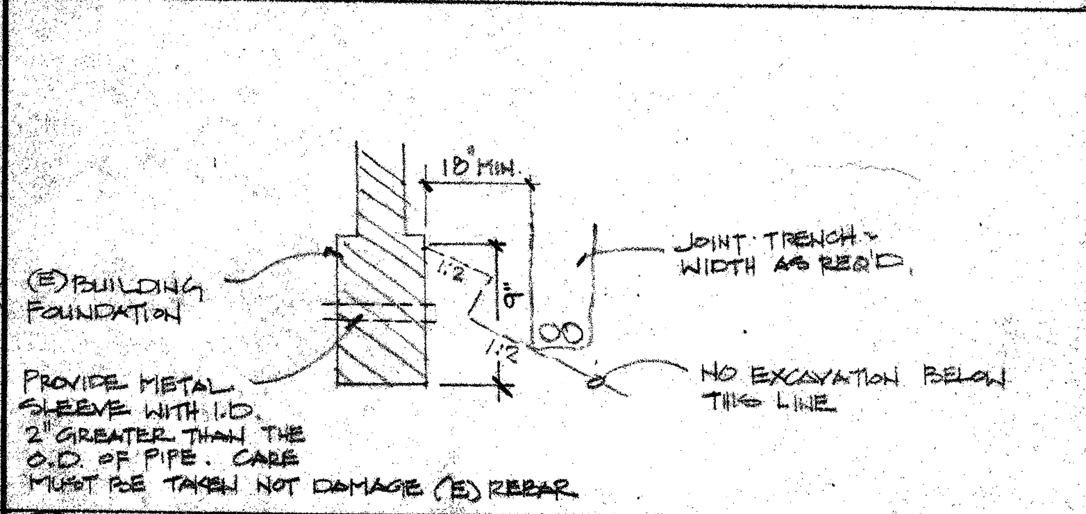
1J JOINT TRENCH
