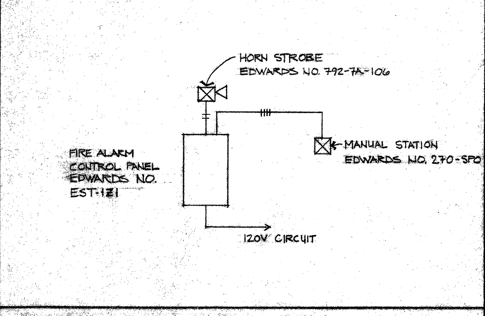
FIRE ALARM RISER DIAGRAM
