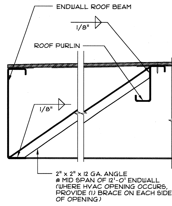
1 ENDWALL DIAGONAL BRACE SCALE: 1/2"=1'-0"
