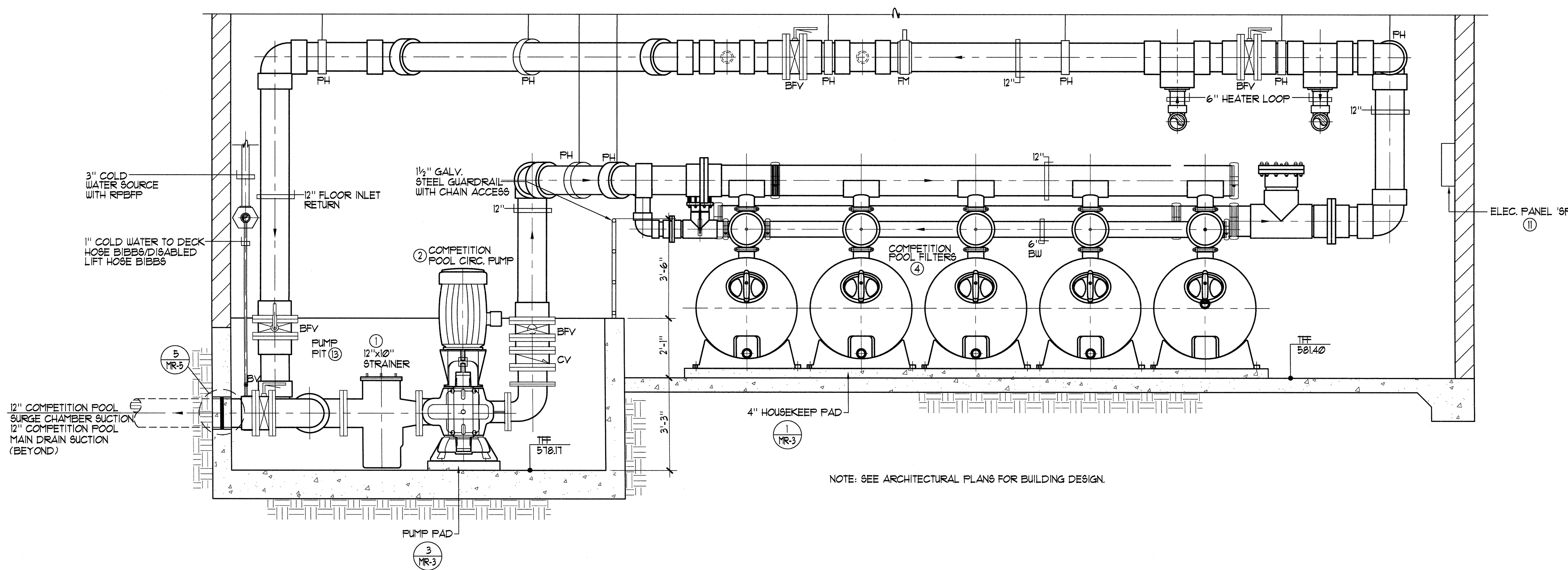
MECHANICAL ROOM SECTION
