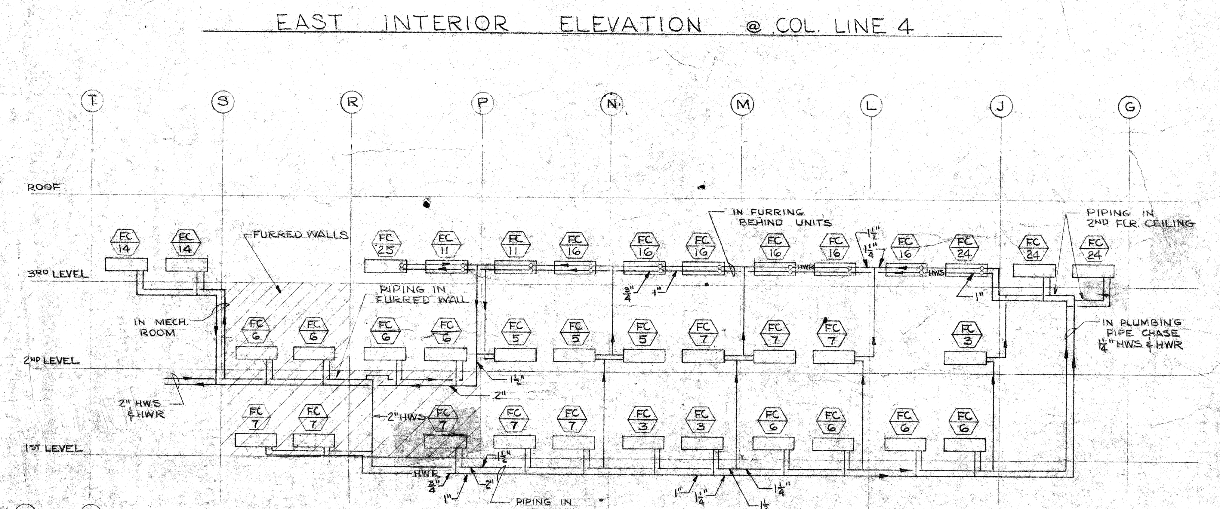
HEATING PIPING RISER DIAGRAMS SCALE: NONE
