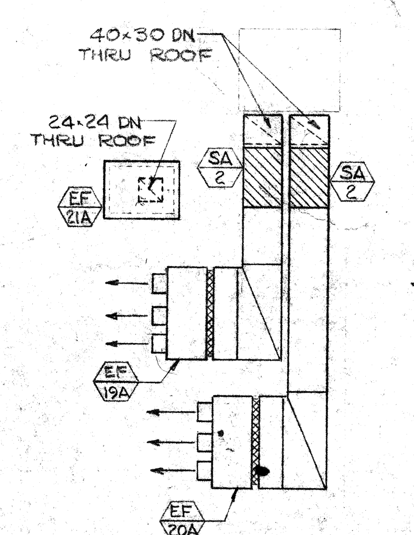
PARTIAL ROOF PLAN SCALE: 1/8" = 1'-0"
