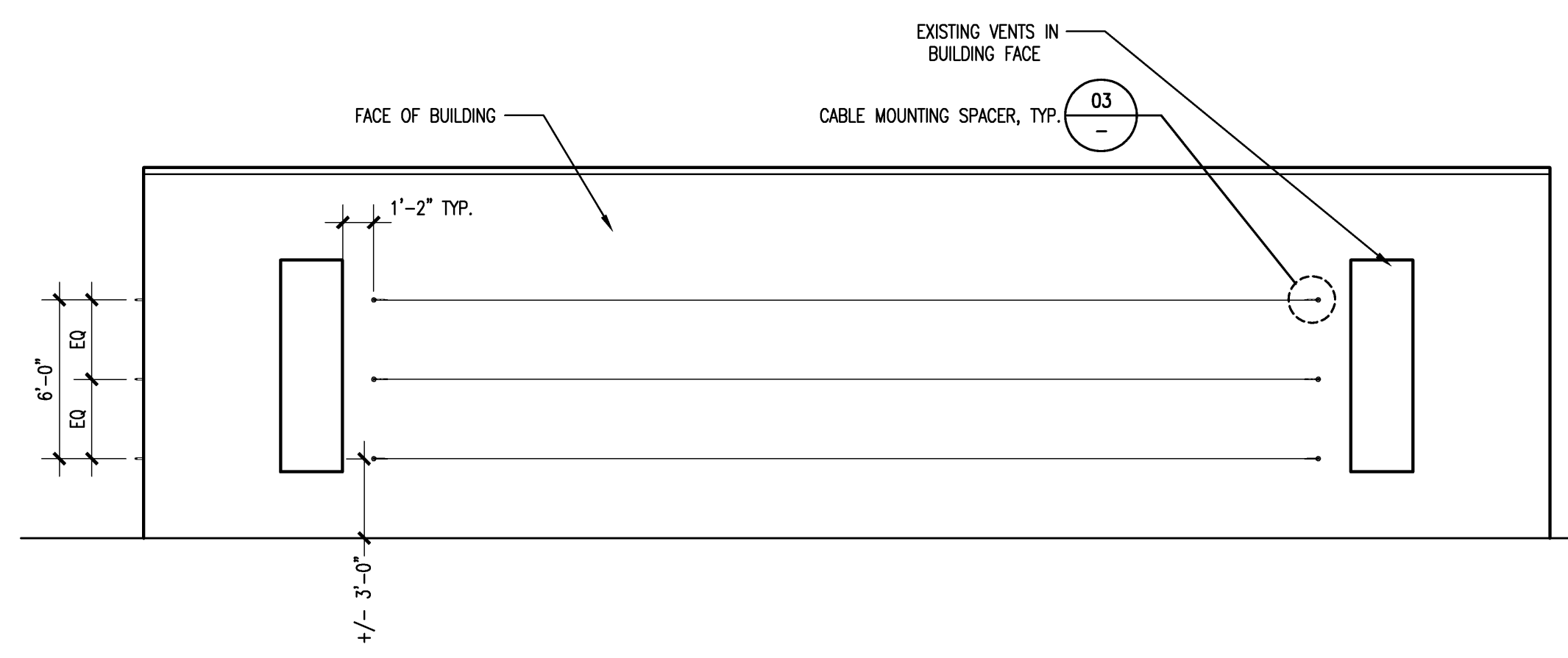
CABLE TRELLIS ELEVATION TYPE 1 3/16" = 1'-0" 01
