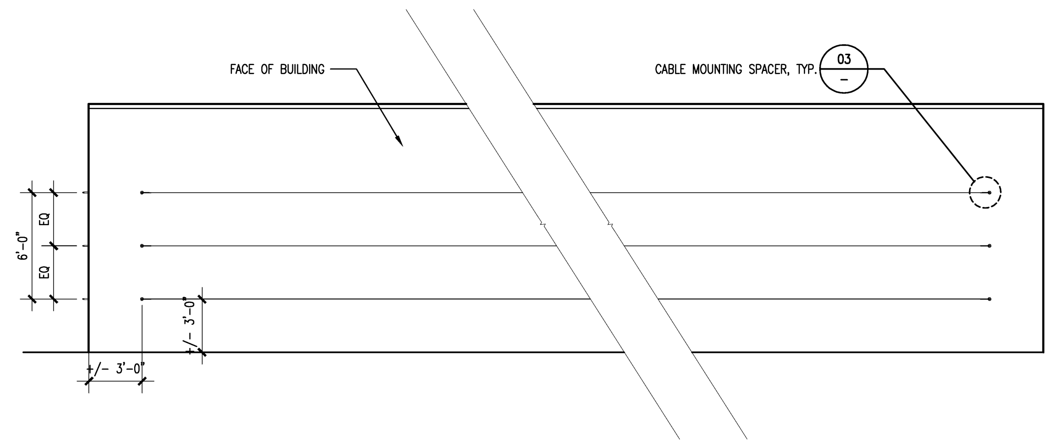
CABLE TRELLIS ELEVATION TYPE 2 3/16" = 1'-0" 02
