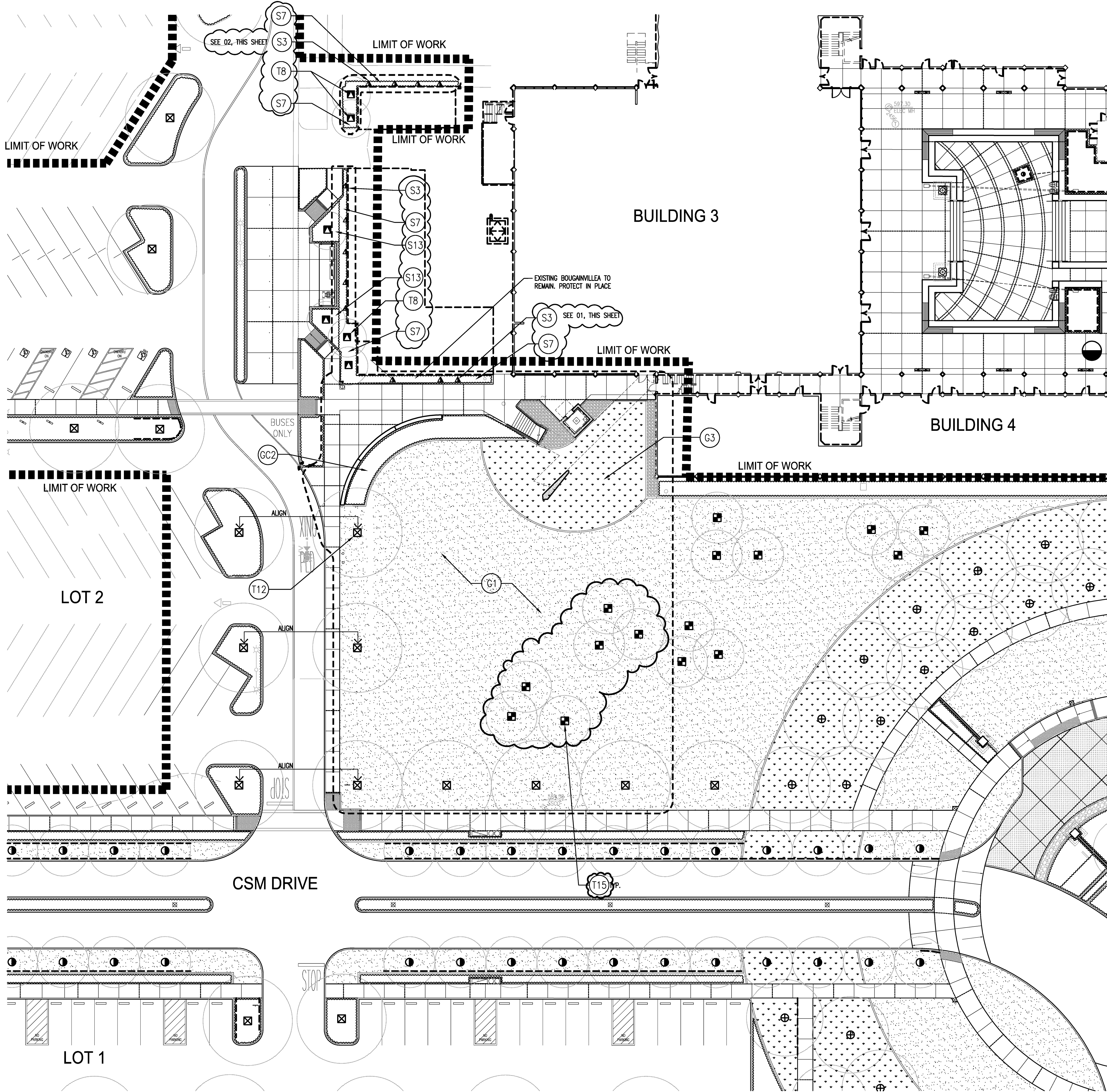
PLANTING PLAN 1" = 20'-0" 01
