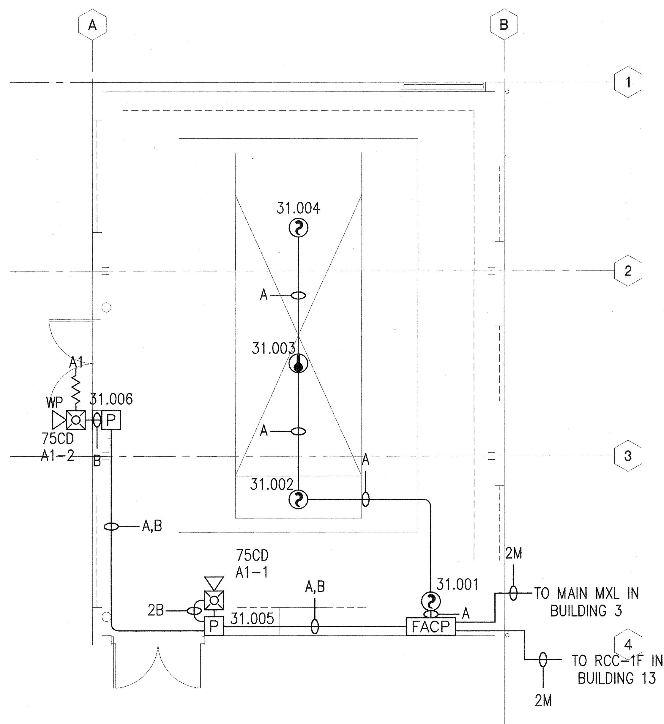
FIRE ALARM PLAN
