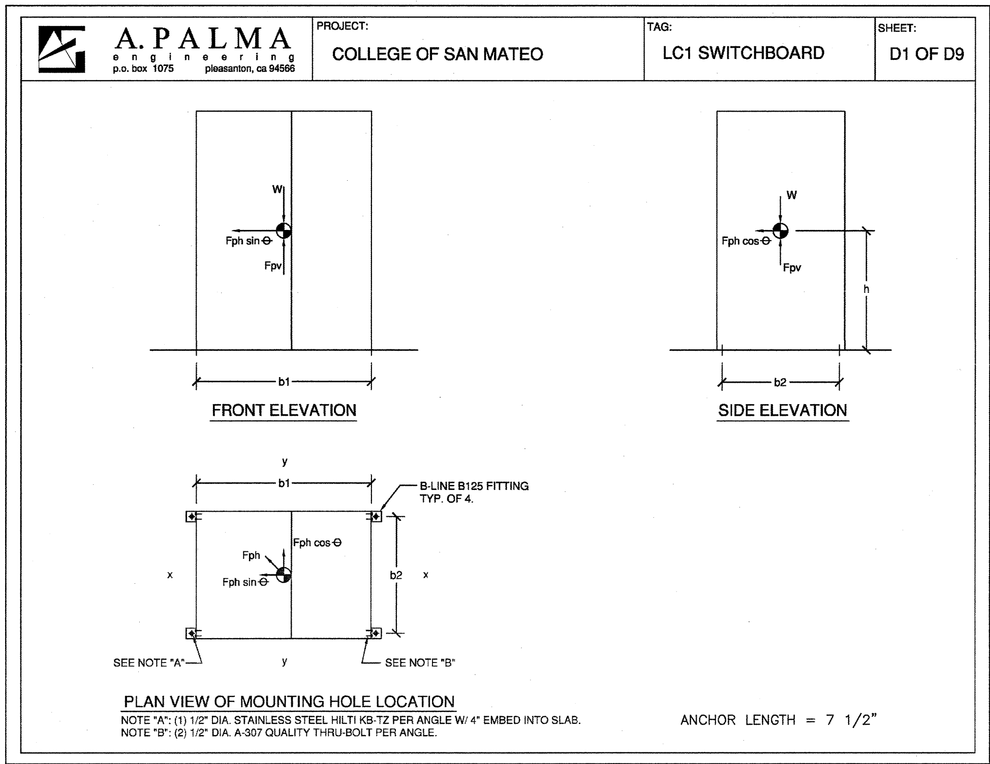
1 LC1 SWITCHBOARD - MOUNTING DETAIL E6.08 SCALE: None
