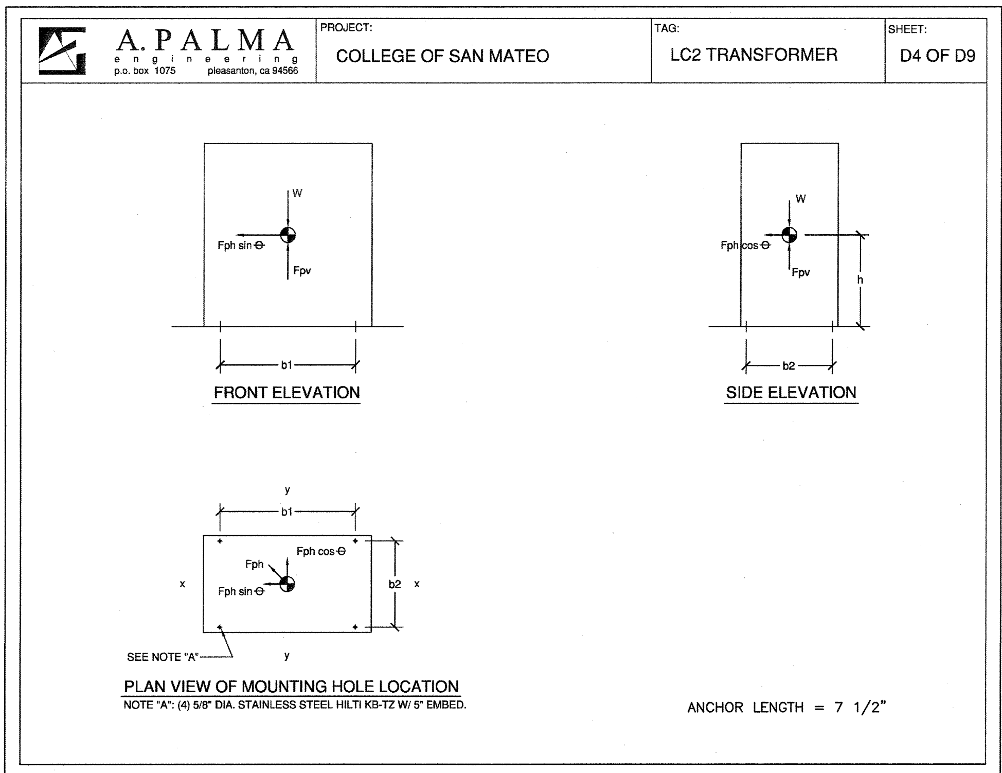
4 LC2 TRANSFORMER - MOUNTING DETAIL E6.08 SCALE: None
