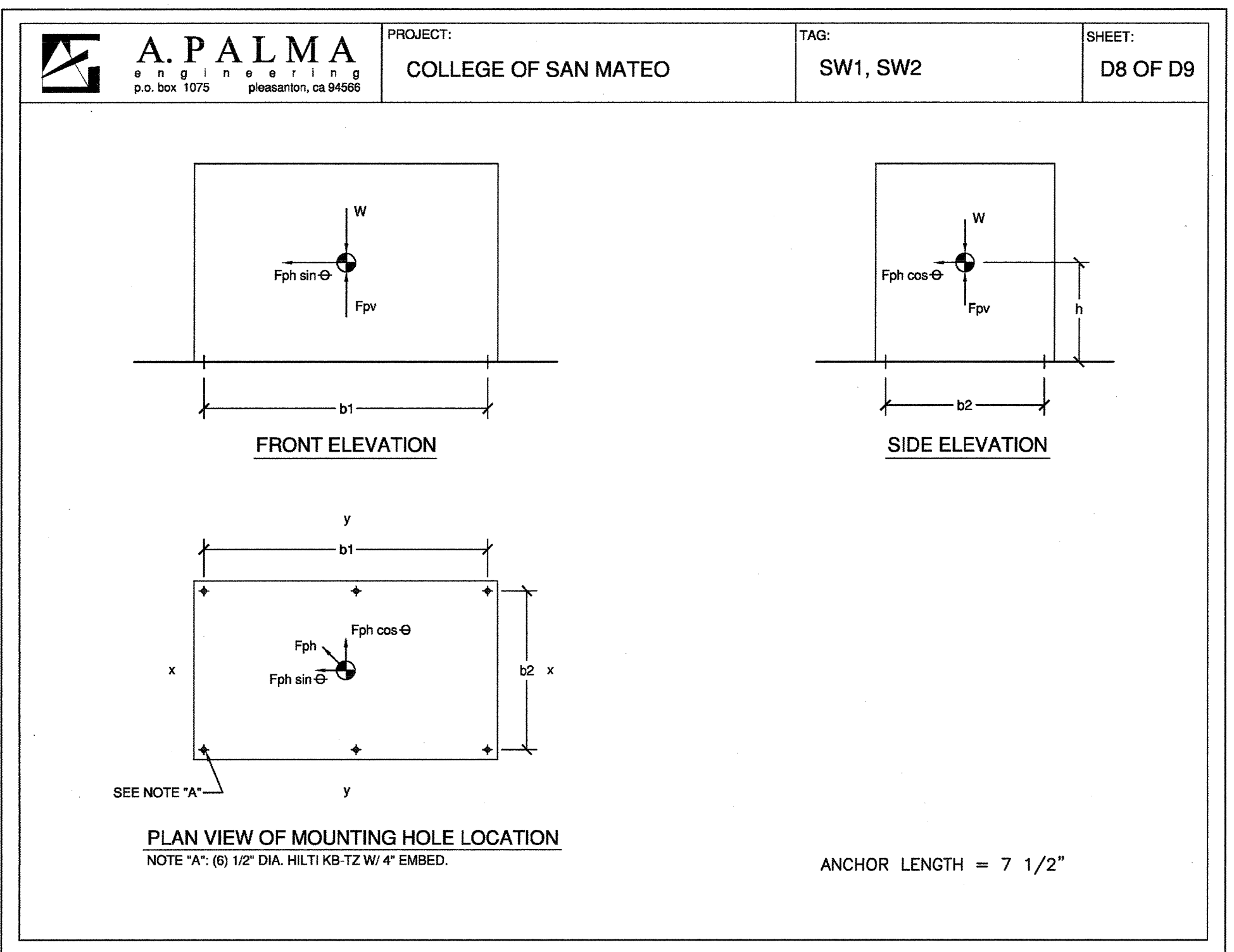
8 SW1 & SW2 SWITCHBOARD - MOUNTING DETAIL E6.08 SCALE: None
