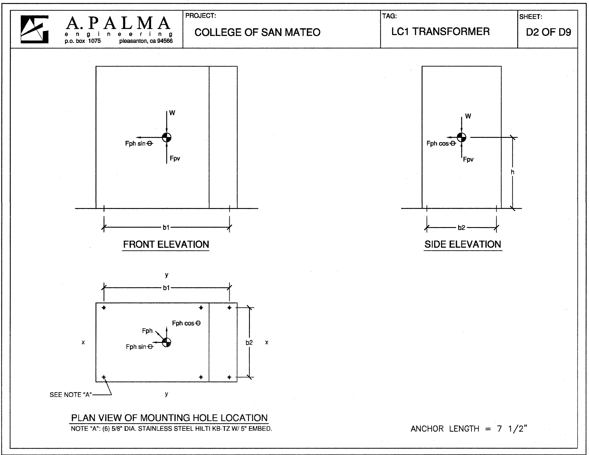
2 LC1 TRANSFORMER - MOUNTING DETAIL E6.08 SCALE: None
