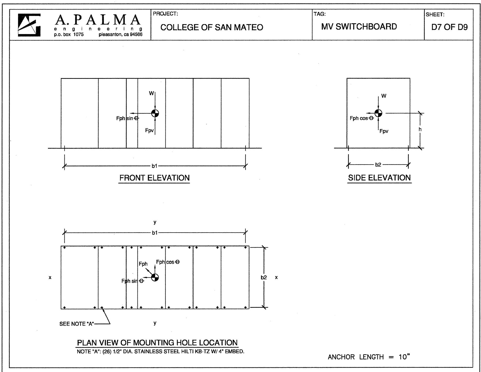
7 MV SWITCHBOARD - MOUNTING DETAIL E6.08 SCALE: None
