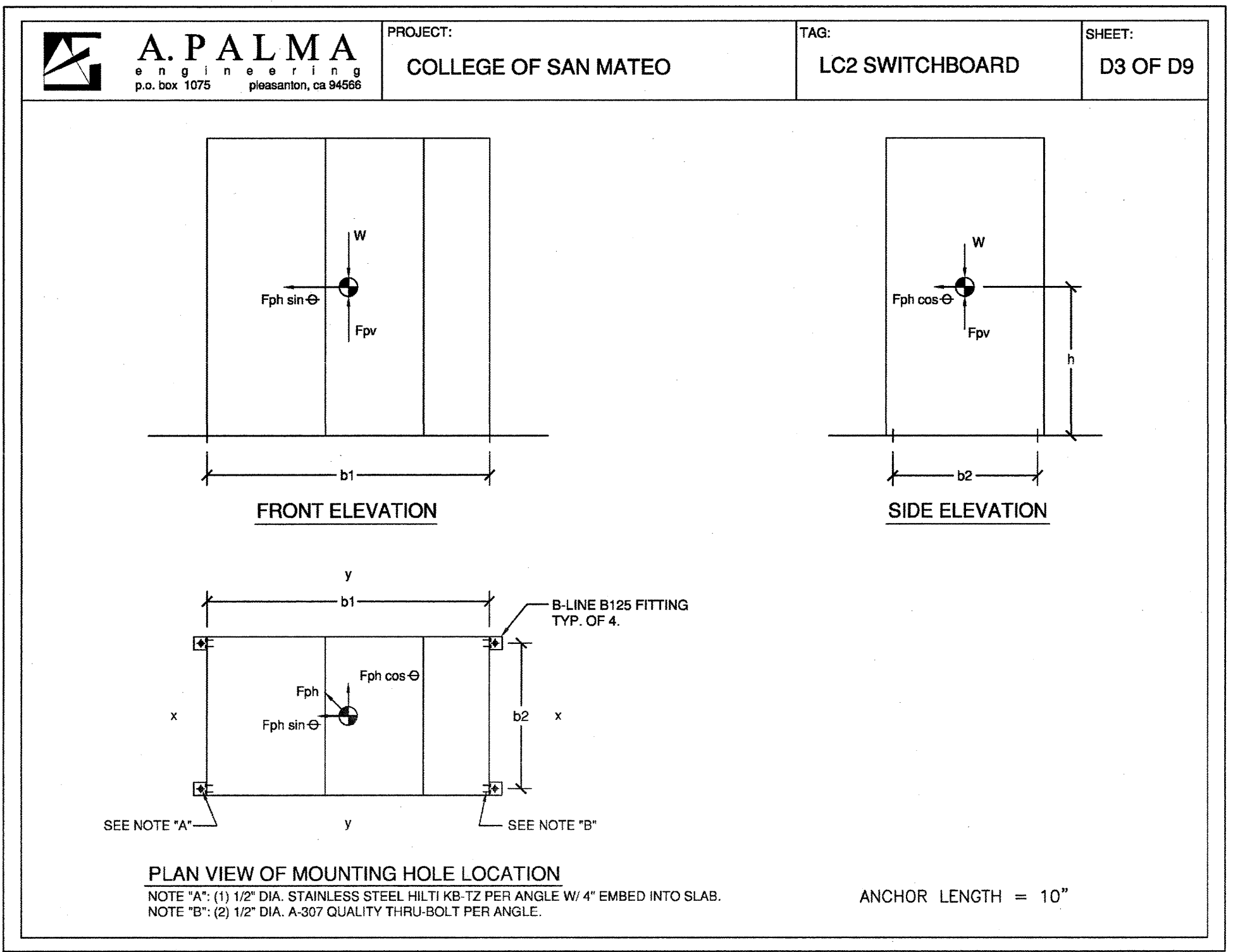
3 LC2 SWITCHBOARD - MOUNTING DETAIL E6.08 SCALE: None
