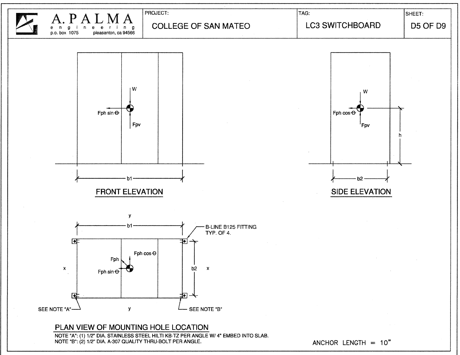
5 LC3 SWITCHBOARD - MOUNTING DETAIL E6.08 SCALE: None
