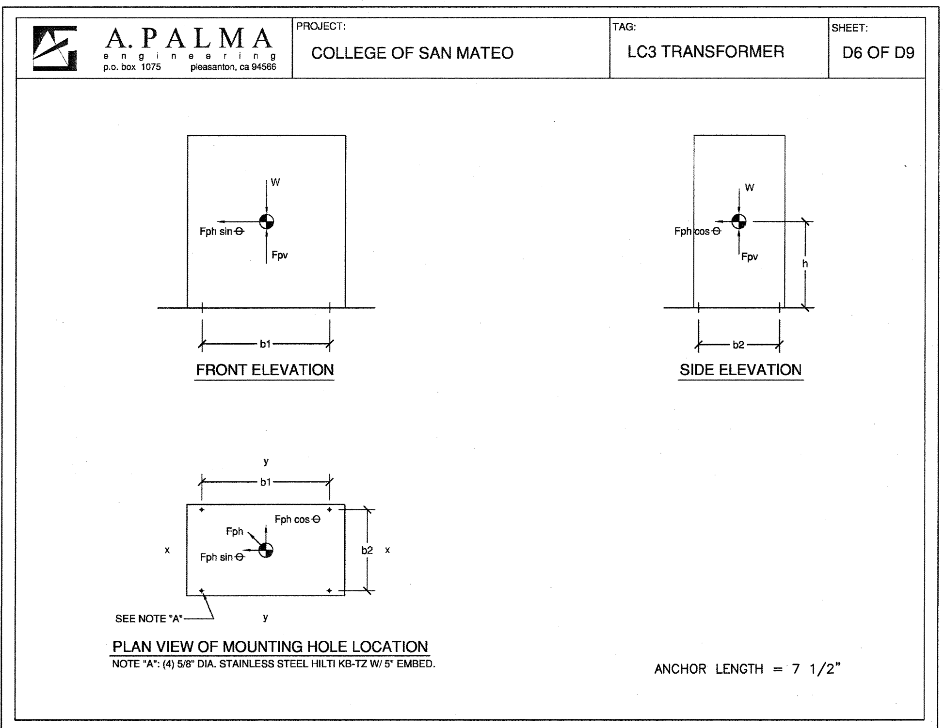
6 LC3 TRANSFORMER - MOUNTING DETAIL E6.08 SCALE: None
