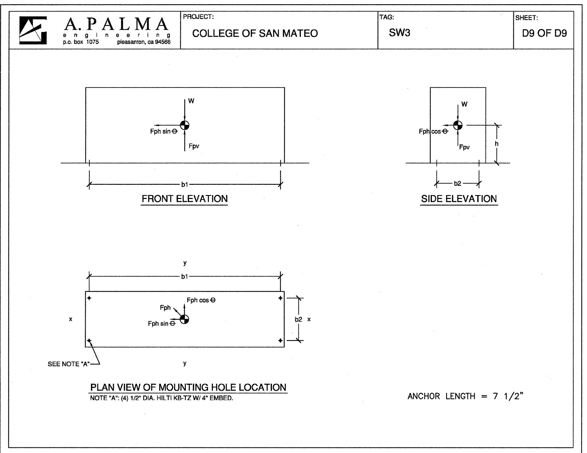
9 SW3 SWITCHBOARD - MOUNTING DETAIL E6.08 SCALE: None
