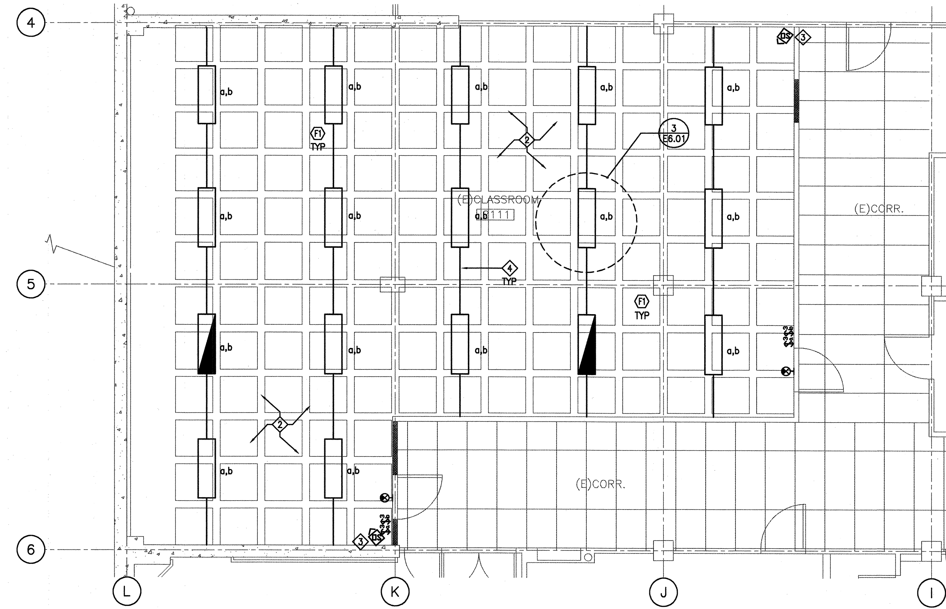
1 ROOM 2111 LIGHTING PLAN 1/4" = 1'-0"
