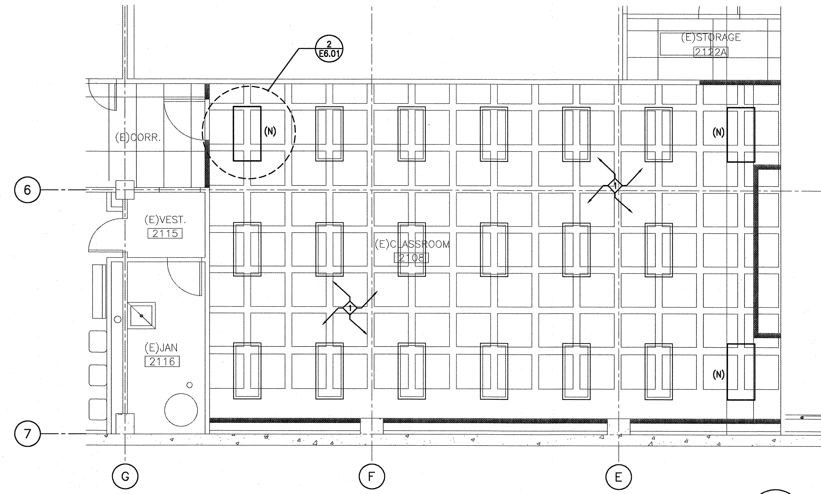
2 ROOF 2108 LIGHTING PLAN 1/4" = 1'-0"
