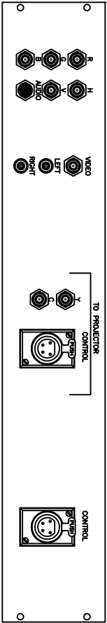
2 AV-7 RACK MOUNTED INPUT PANEL
