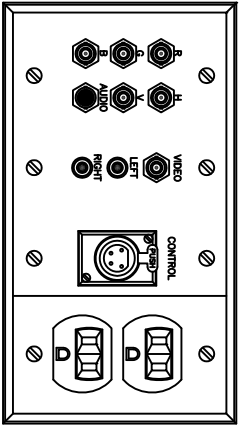
1 AV-7 LEFT, CENTER, RIGHT INPUT PLATE (TYPICAL OF 3) ALL CONNECTORS RECESSED
