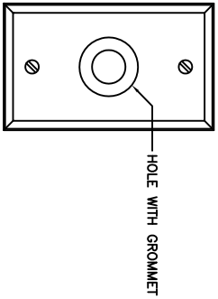
3 AV-7 LOUDSPEAKER PLATE (FRONT/LEFT/RIGHT)
