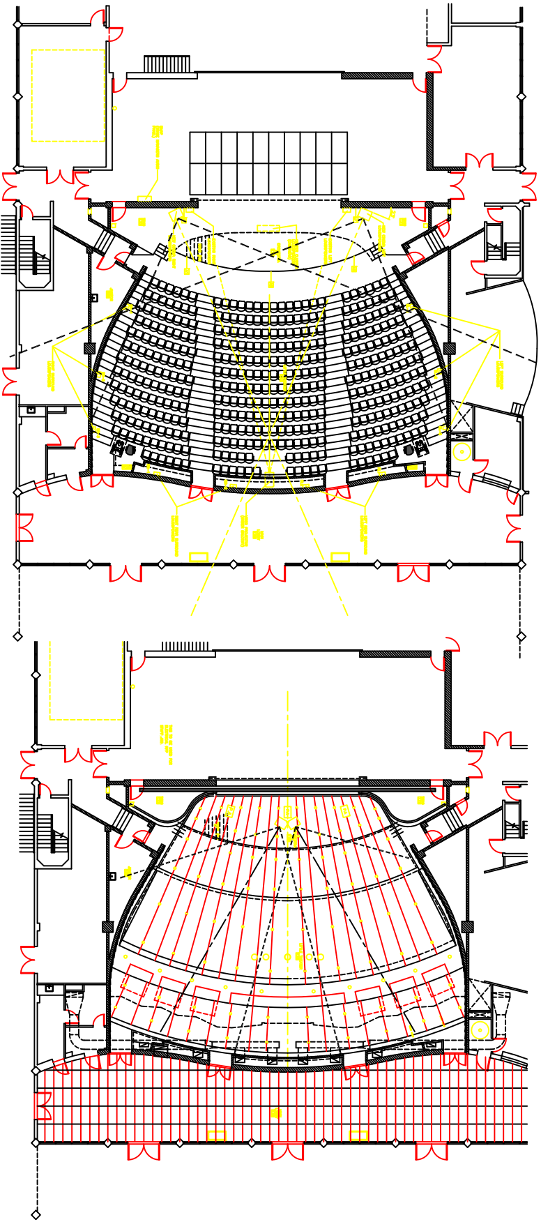
1 LEFT/RIGHT LOUDSPEAKER COVERAGE DETAIL
