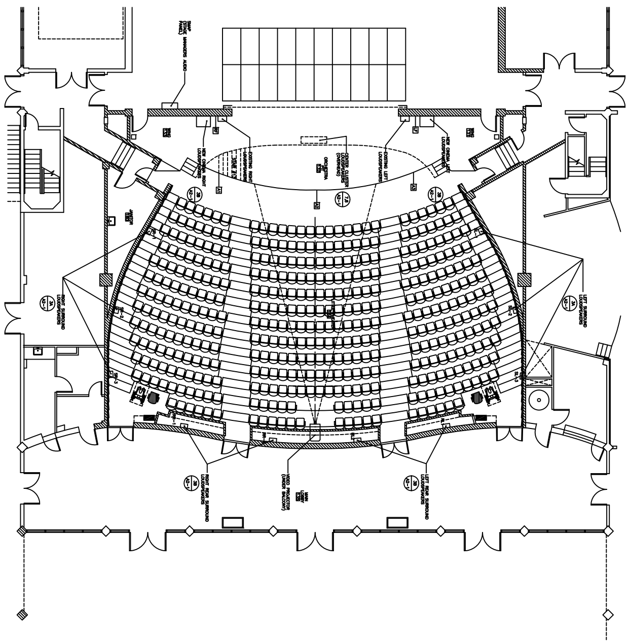
1 AV-2 AUDIOVISUAL FLOOR PLAN
