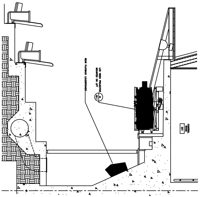
1 AV-1 PROJECTOR MOUNTING AND LOCATION DETAIL
