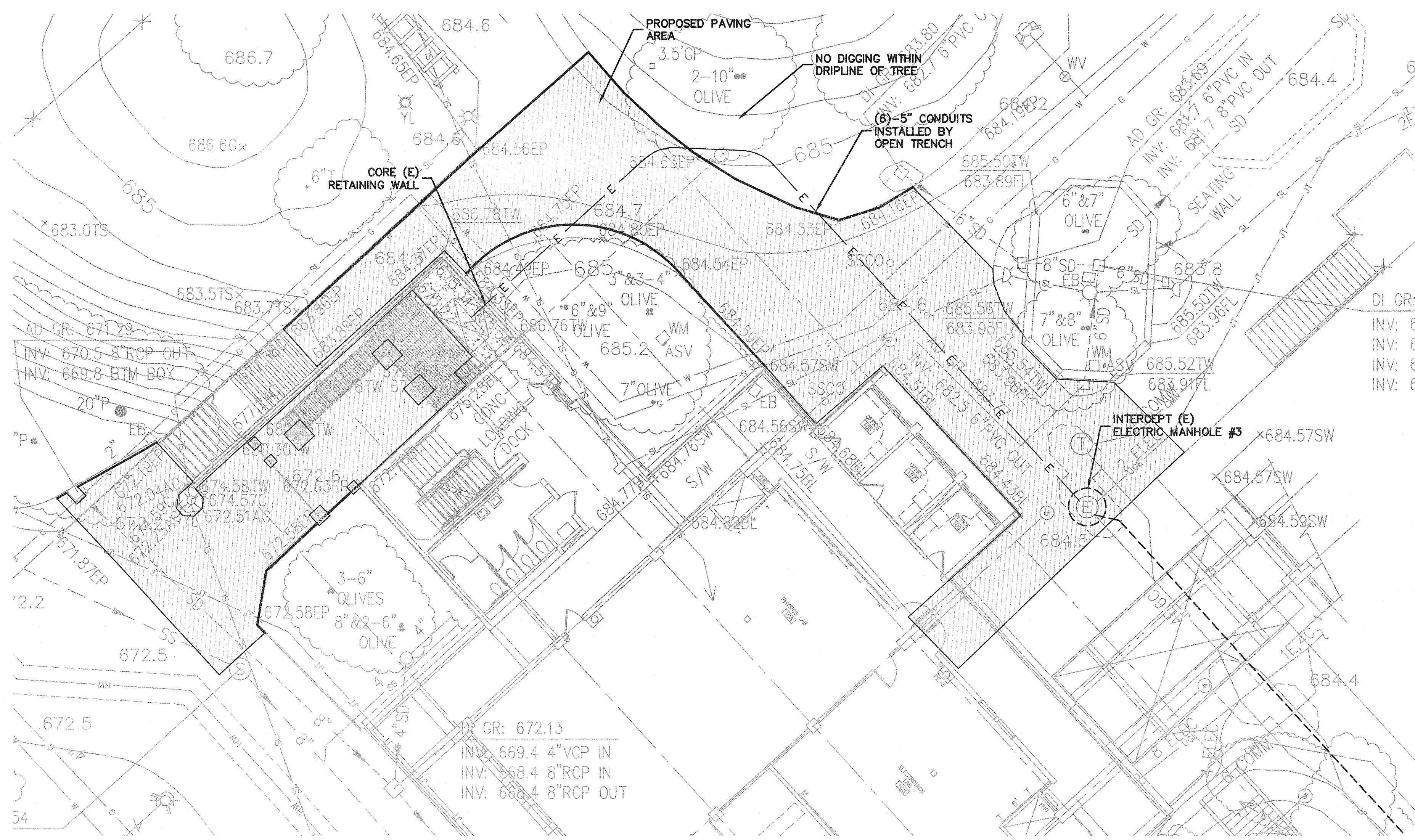
1 BUILDING 16 AREA SCALE: 1" = 10'
