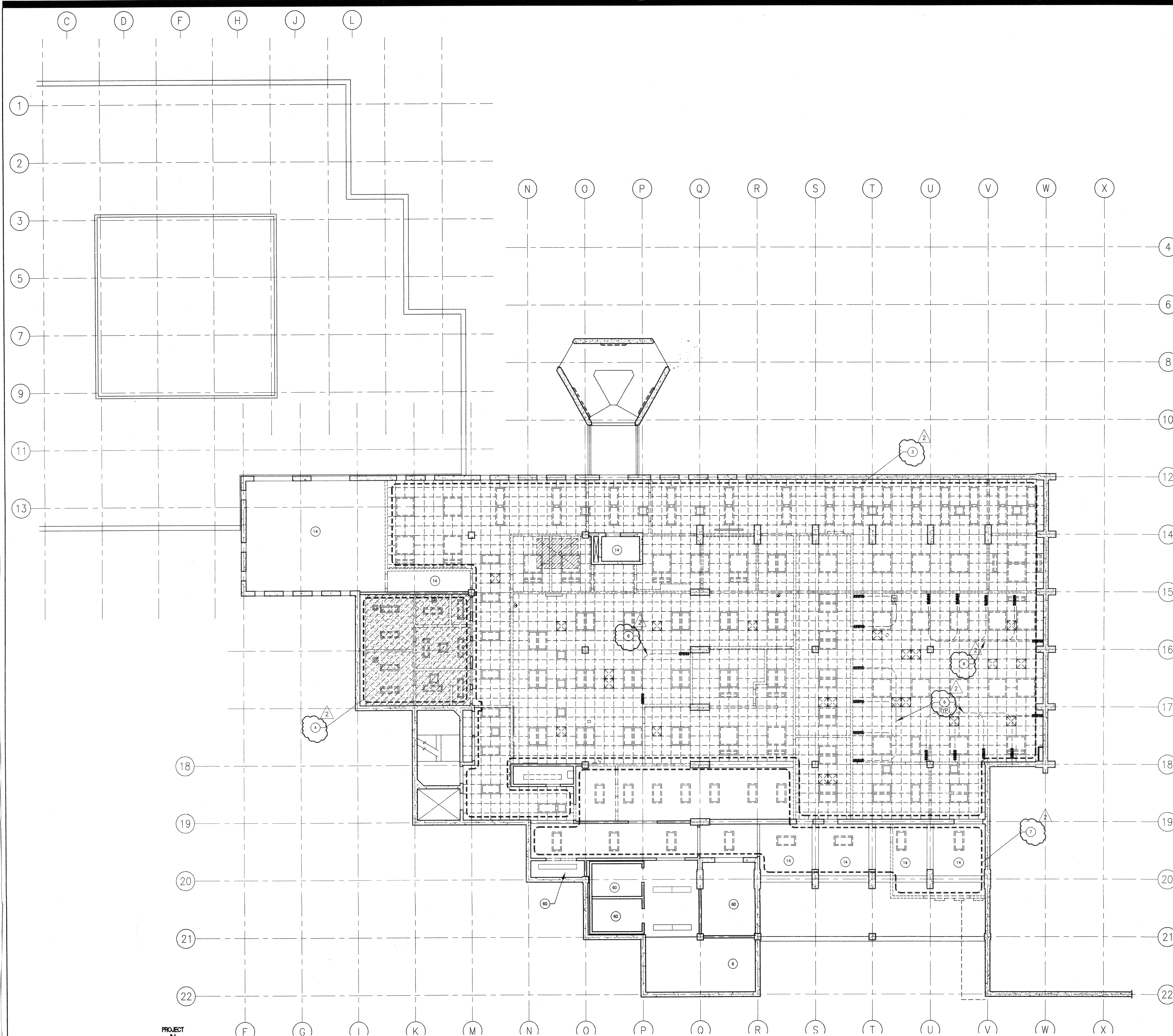
SECOND FLOOR REFLECTED CEILING DEMO PLAN
