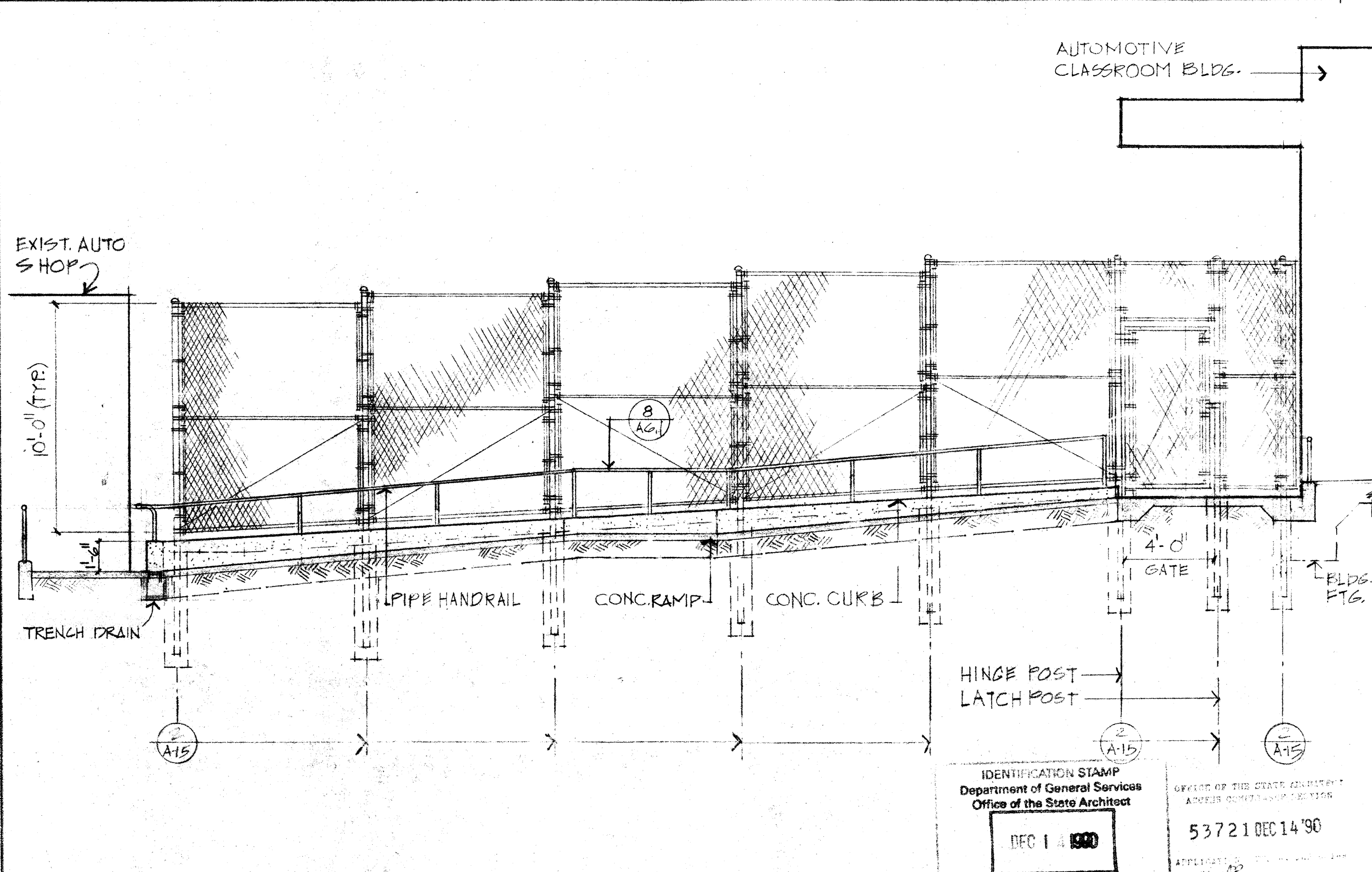
FENCE NORTH ELEVATION
