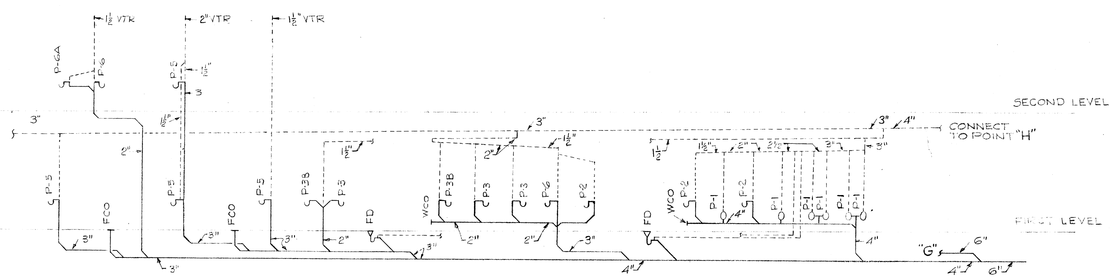
SOIL, WASTE & VENT PIPING DIAGRAM ROOMS 1, 3, 11, 12, 14 & 130A NO SCALE
