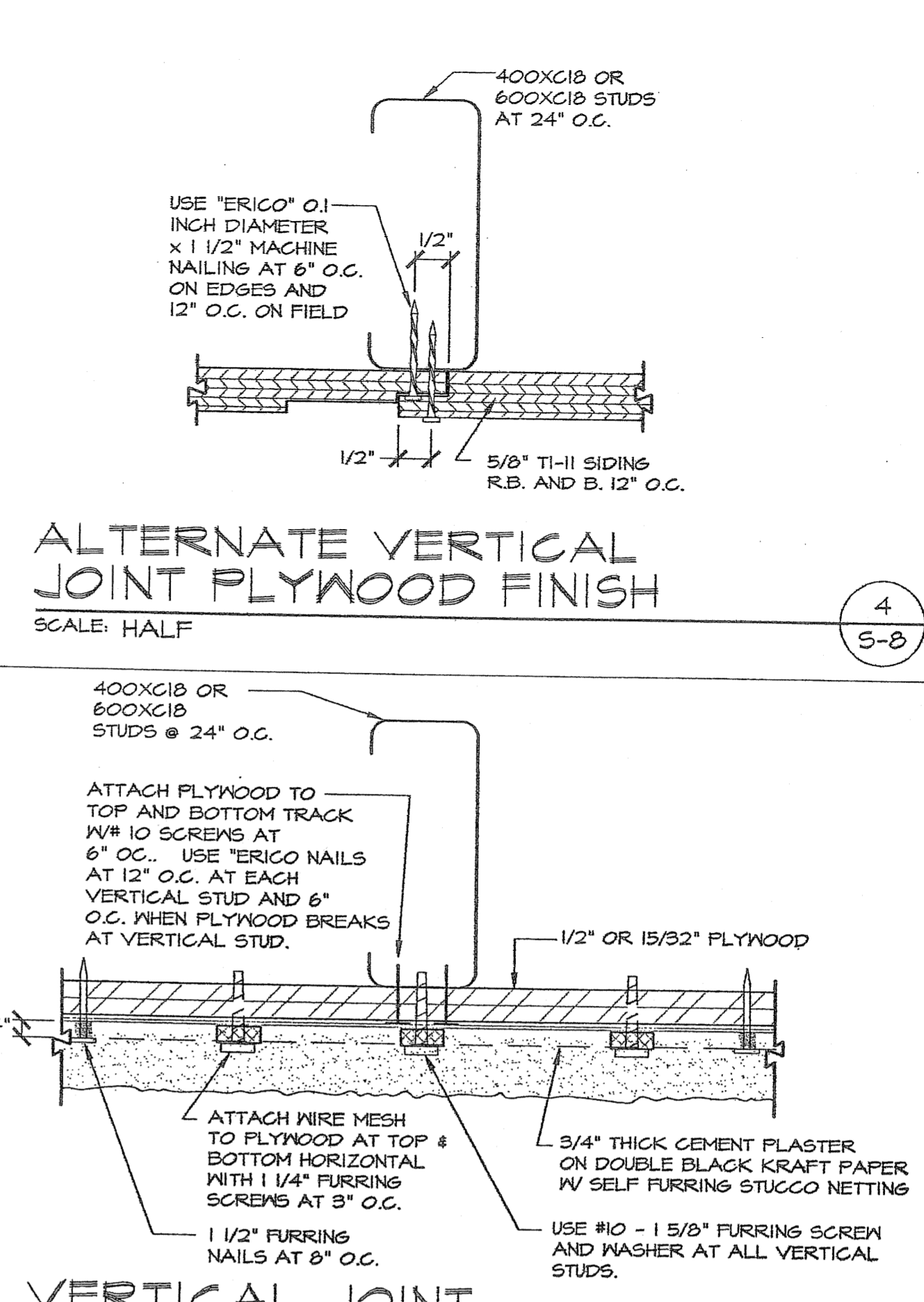
VERTICAL JOINT STUCCO FINISH SCALE: HALF
