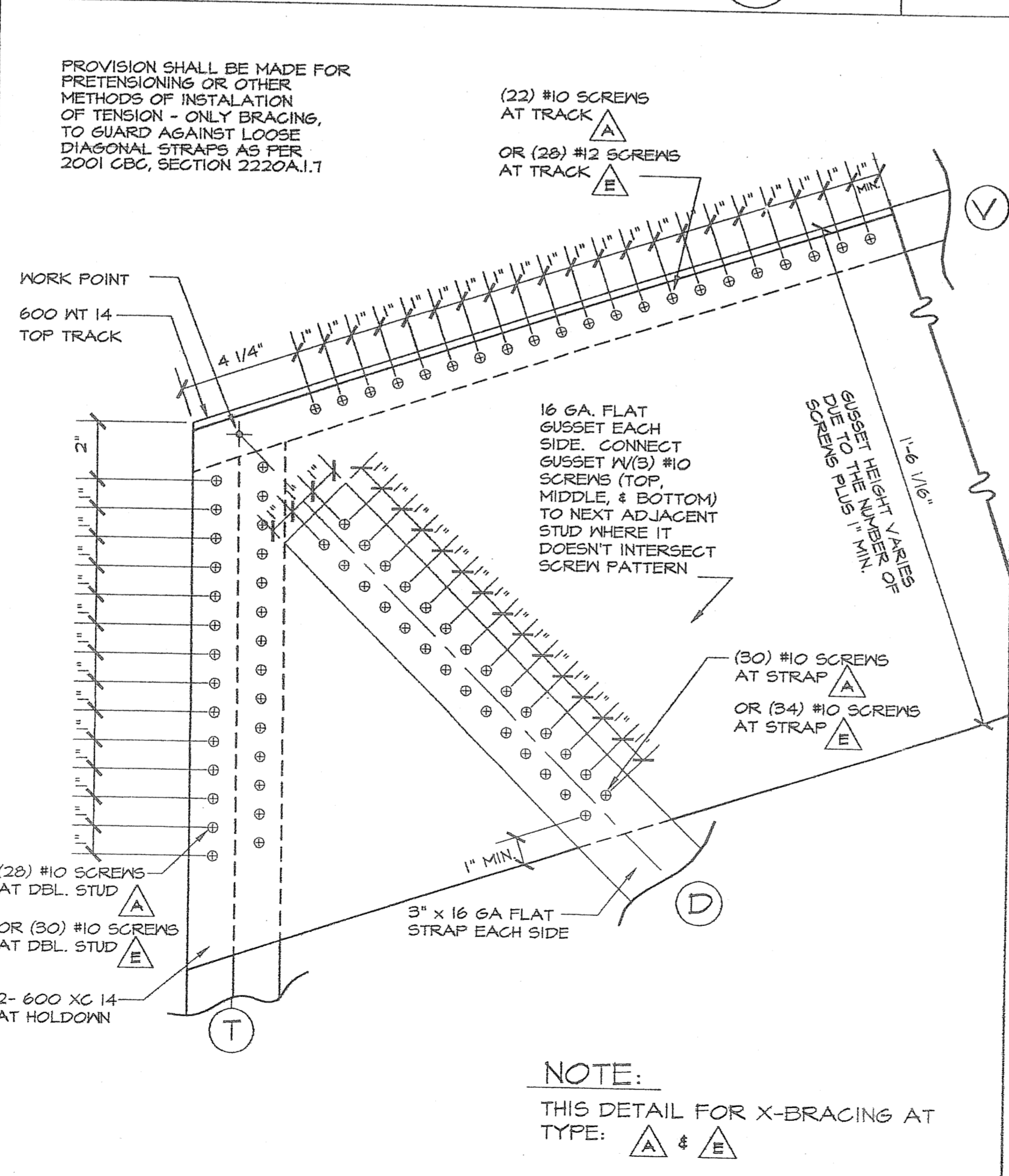
TOP GUSSET AT RAKED WALL X-BRACING SCALE: 3" = 1'-0"
