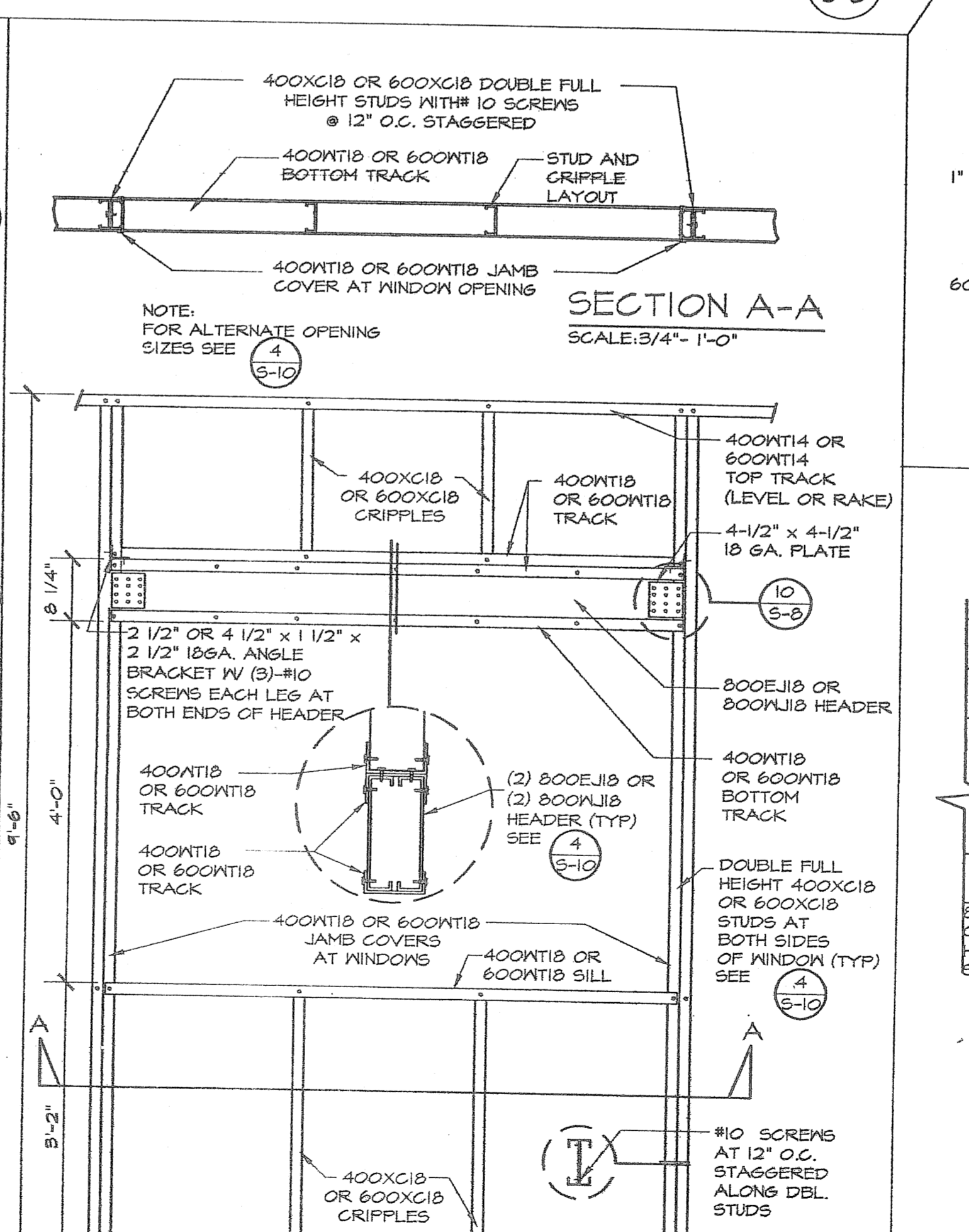
TYPICAL HEADER & SILL SCALE: 3/4" = 1'-0"
