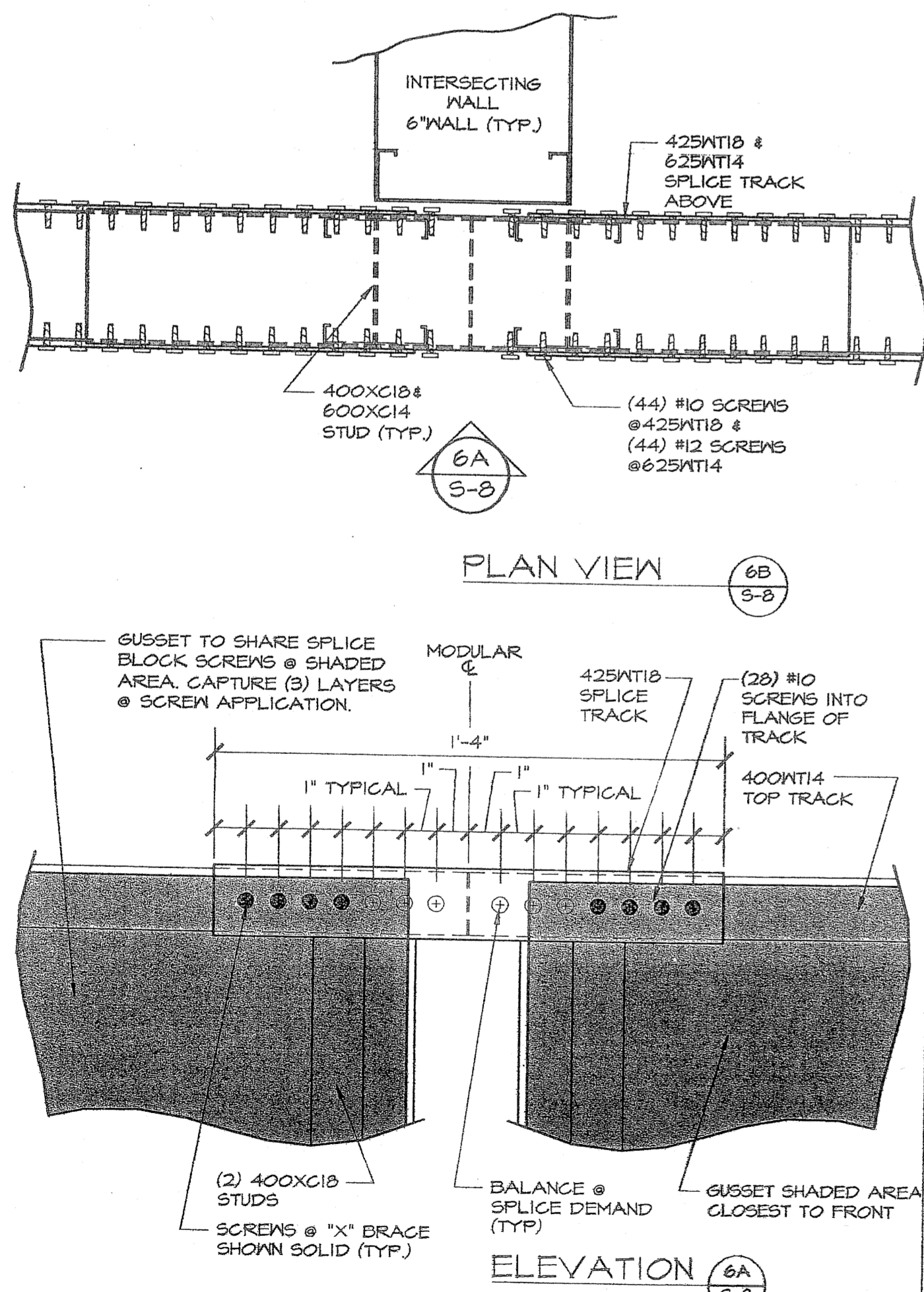
TOP TRACK MODULAR SPLICE SCALE: 3" = 1'-0"
