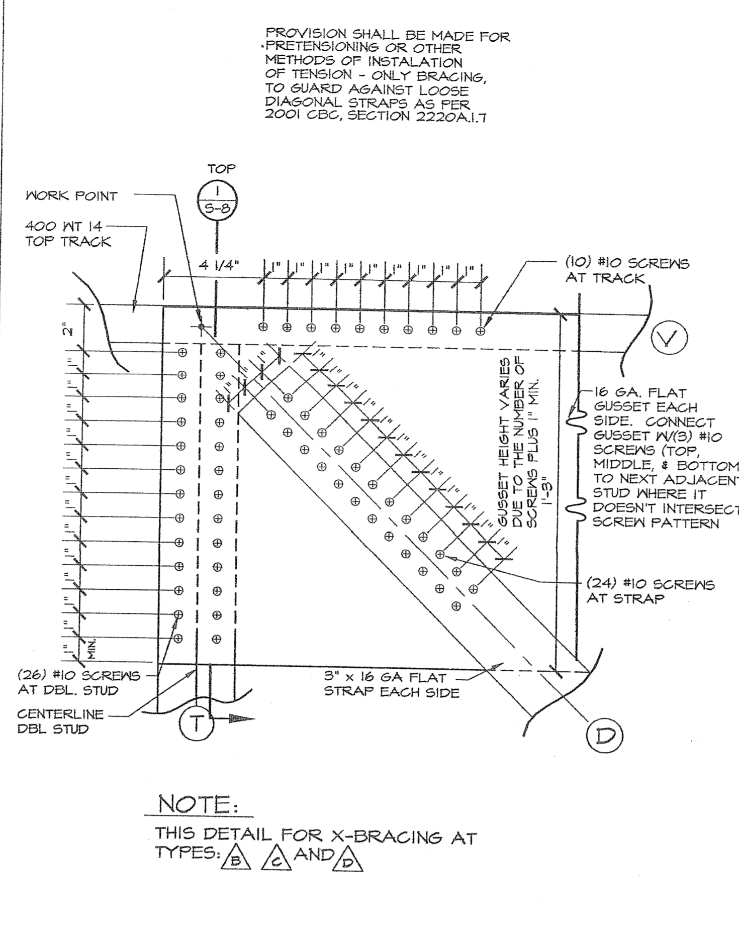
TOP GUSSET AT STRAIGHT WALL X-BRACING SCALE: 3" = 1'-0"
