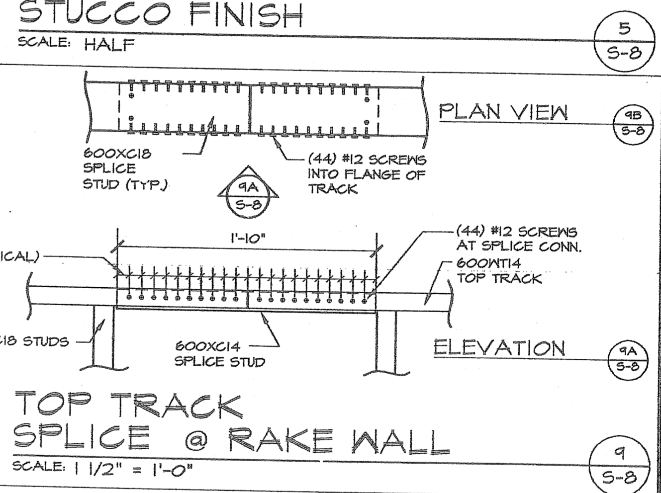
TOP TRACK SPLICE @ RAKE WALL SCALE: 1 1/2" = 1'-0"
