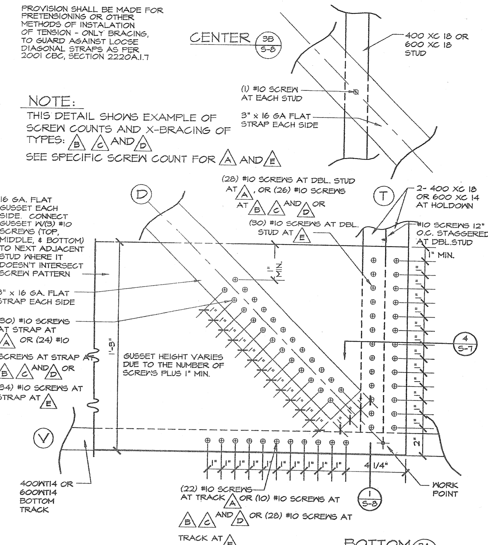
TYPICAL CENTER & BOTTOM GUSSET AT X-BRACING SCALE: 3" = 1'-0"
