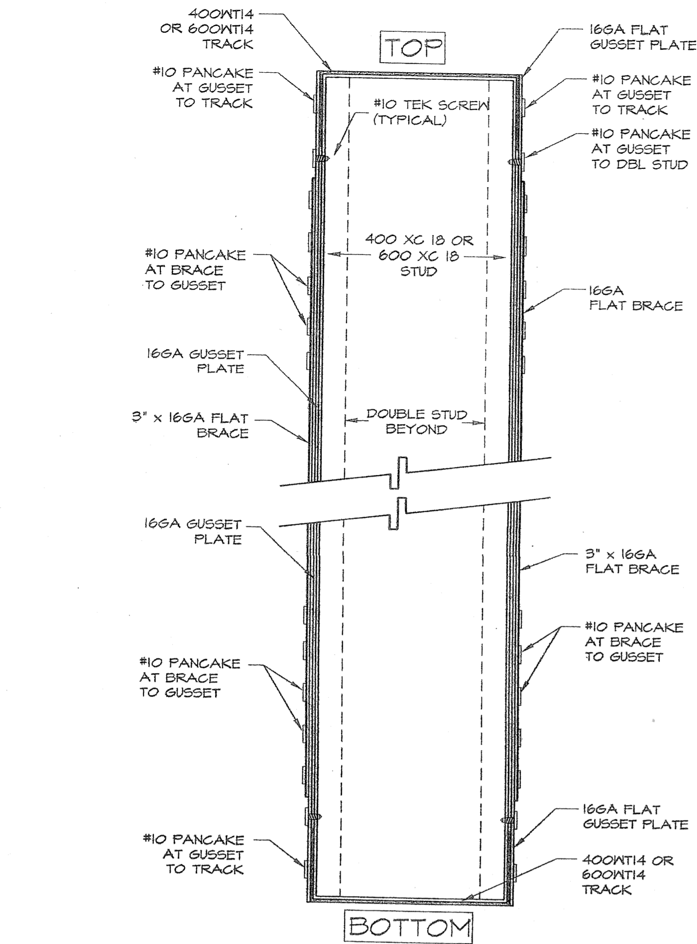
GUSSET AND CROSS BRACING SCALE: HALF
