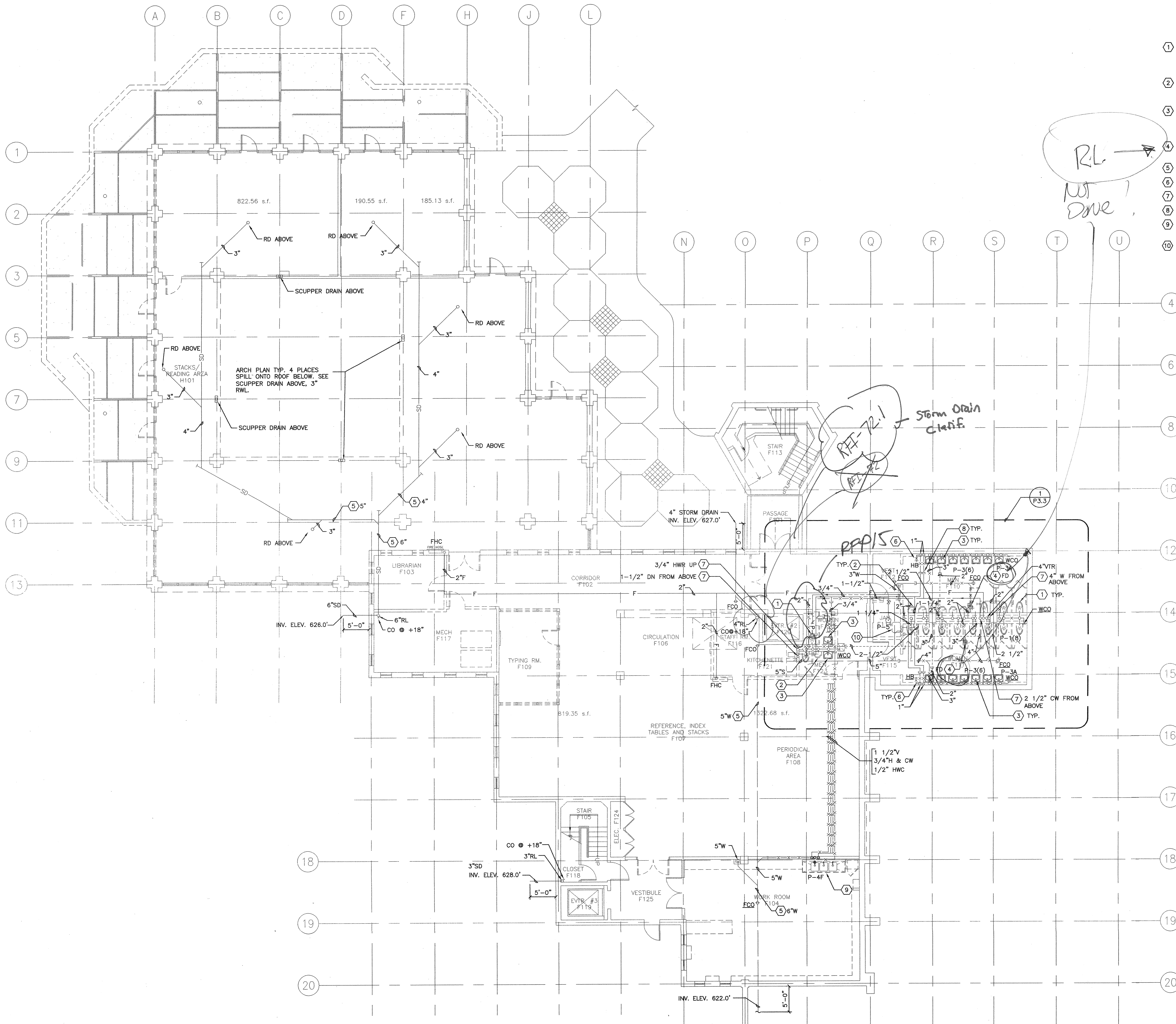
1 FIRST FLOOR DEMOLITION PLAN - PLUMBING 0 4' 8' 16' SCALE: 1/8"=1'-0"
