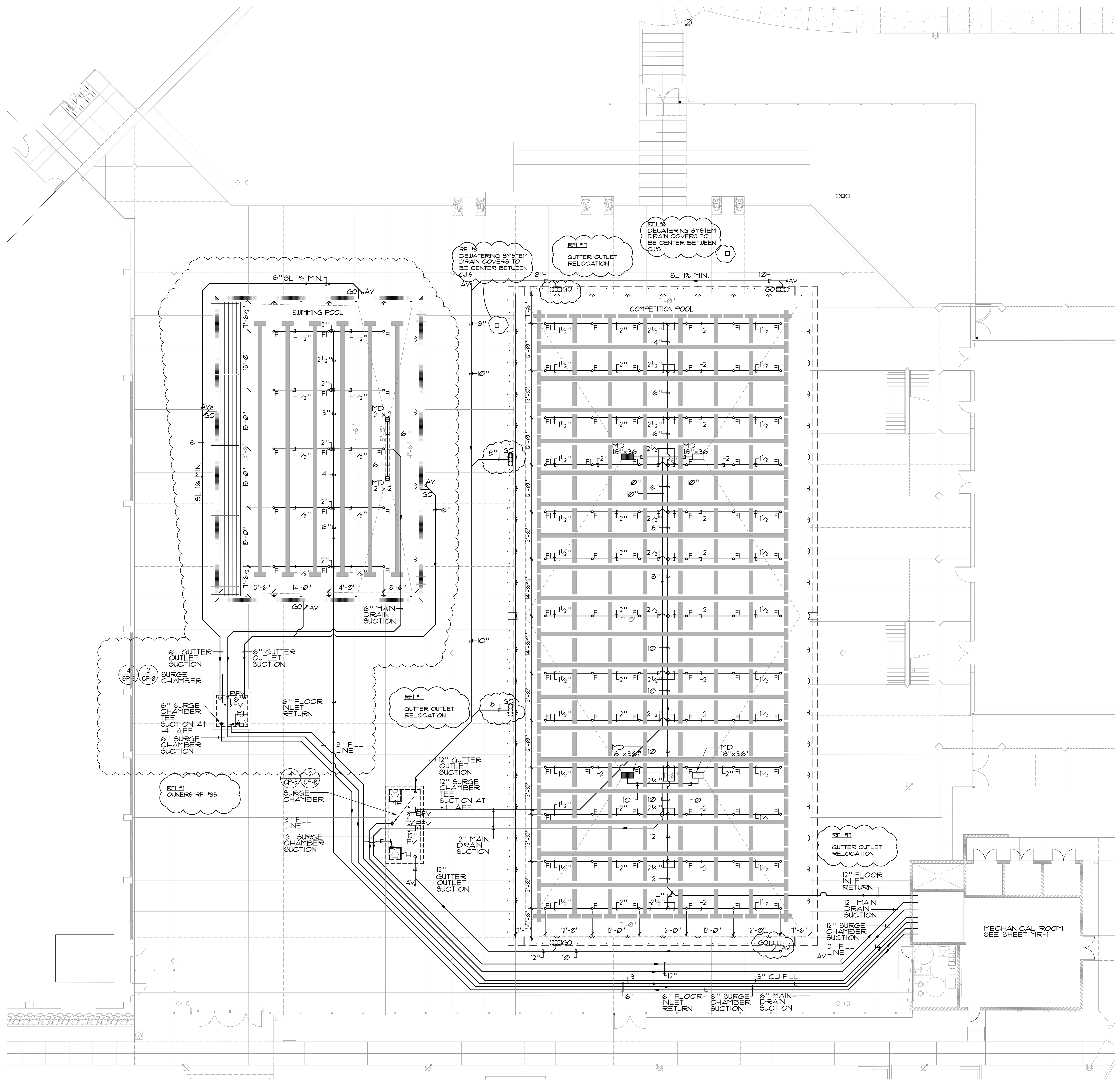
COMPETITION POOL/SWIMMING POOL PIPING PLAN 1"=10'-0"
