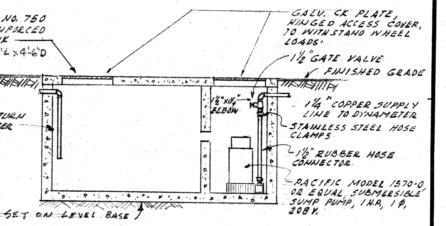
DETAIL OF COOLING WATER STORAGE TANK SCALE: 1/2" = 1'-0"
