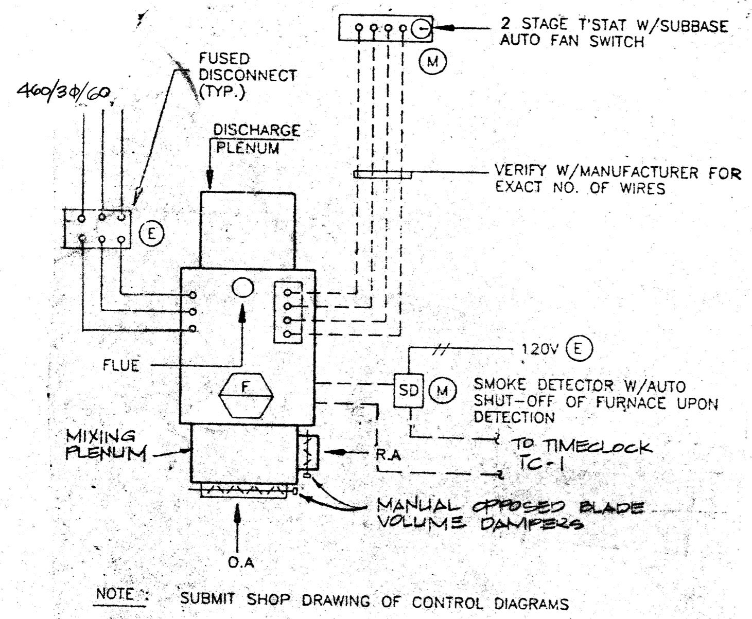
FURNACE
