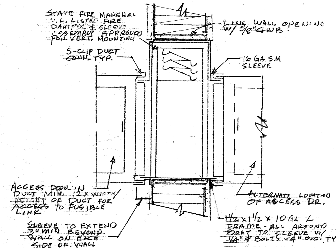
WALL FIRE DAMPER NTS 5
