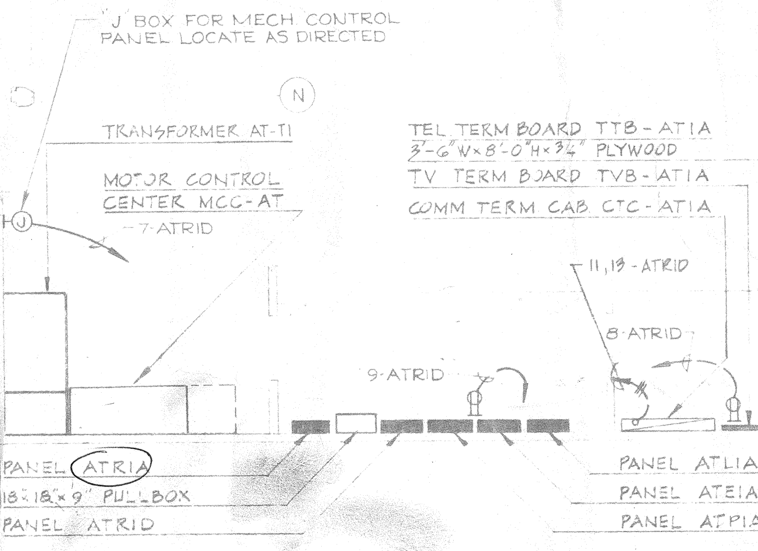
ELECTRIC CLOSET #377A SCALE 1/4"=1'-0"
