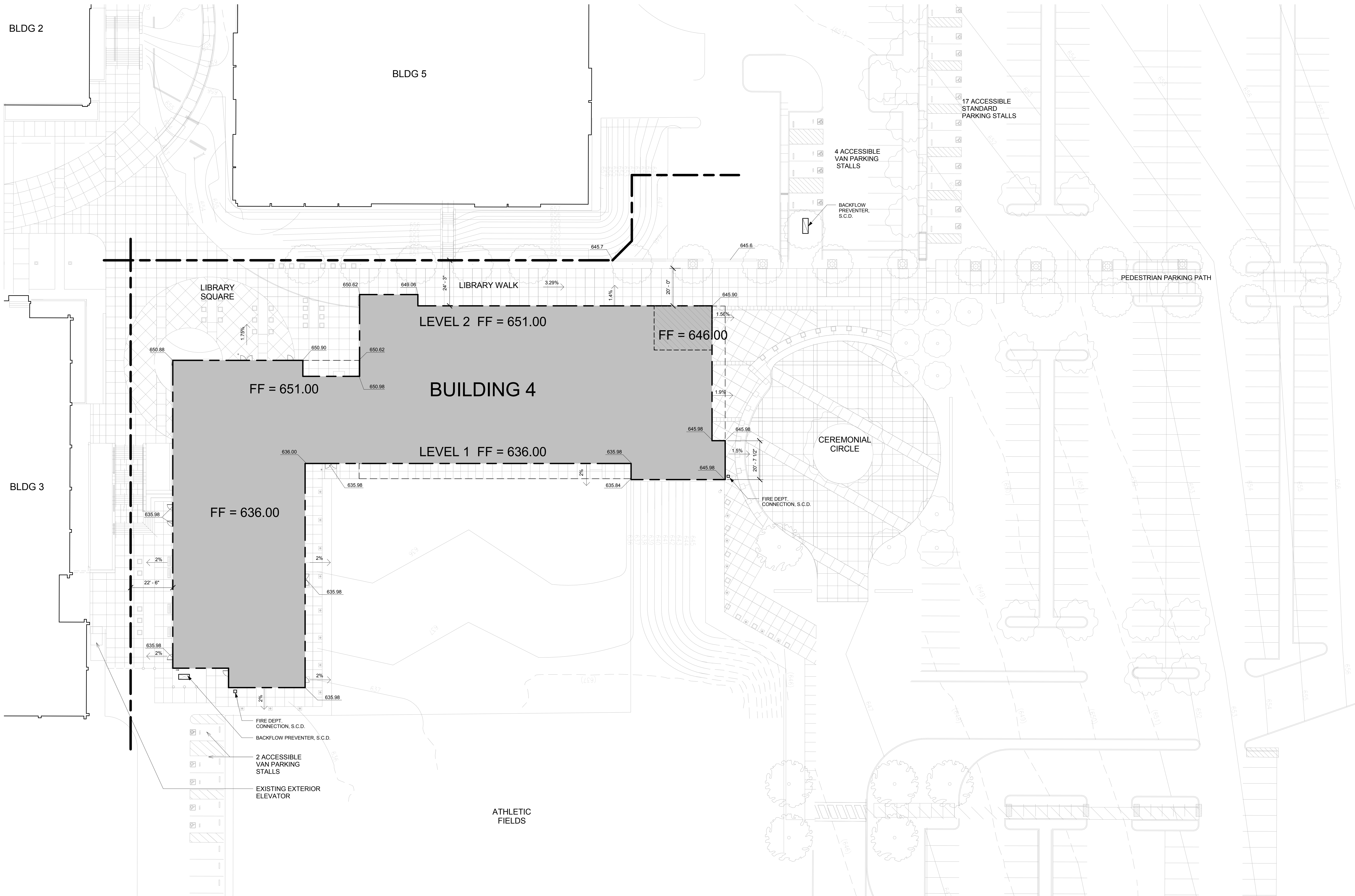
1 SITEPLAN 1" = 20'-0"
