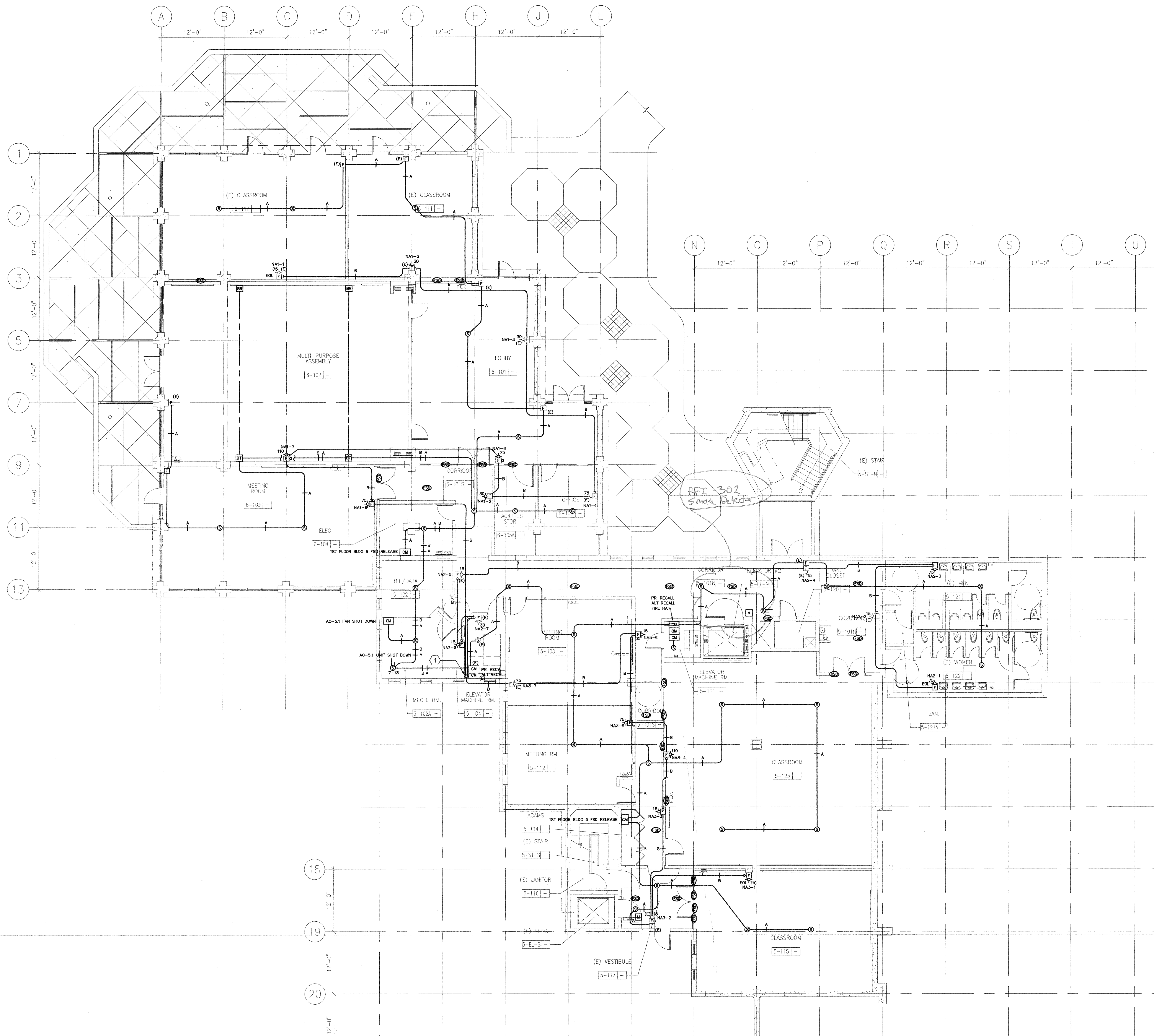
1 FIRE ALARM PLAN - FIRST FLOOR SCALE: 1/8"=1'-0"
