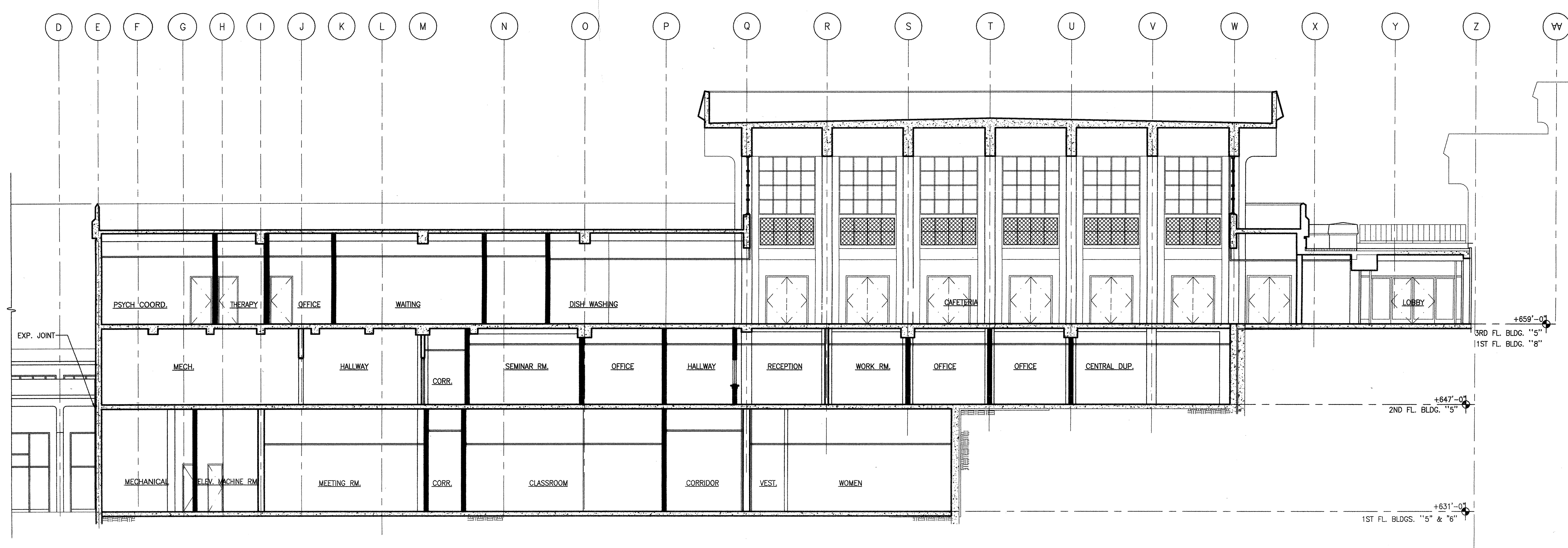
BUILDING SECTION 1 SCALE 1/4" = 1'-0" 0 4 8'
