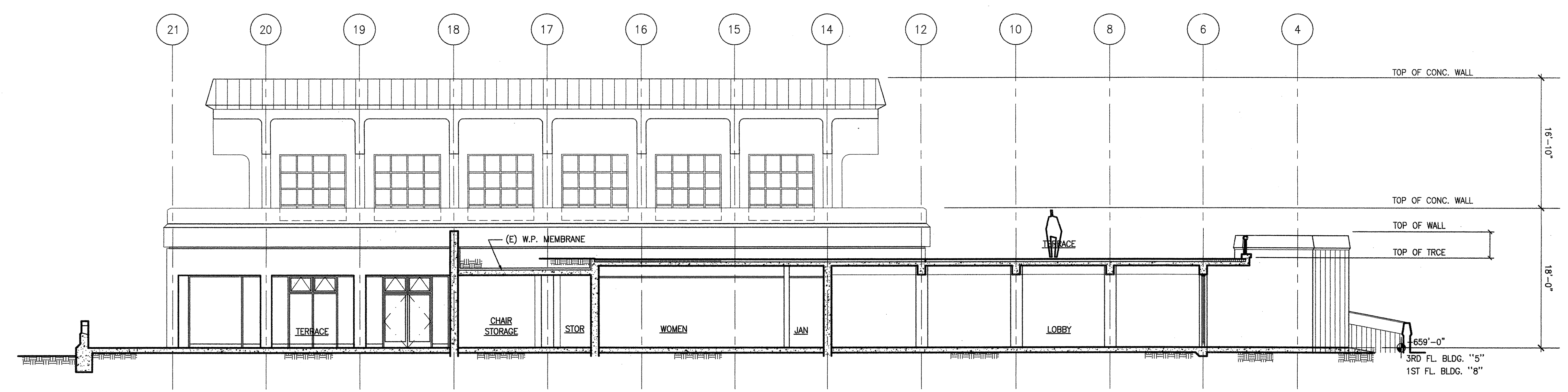
BUILDING SECTION 2 SCALE 1/4" = 1'-0" 0 4 8'
