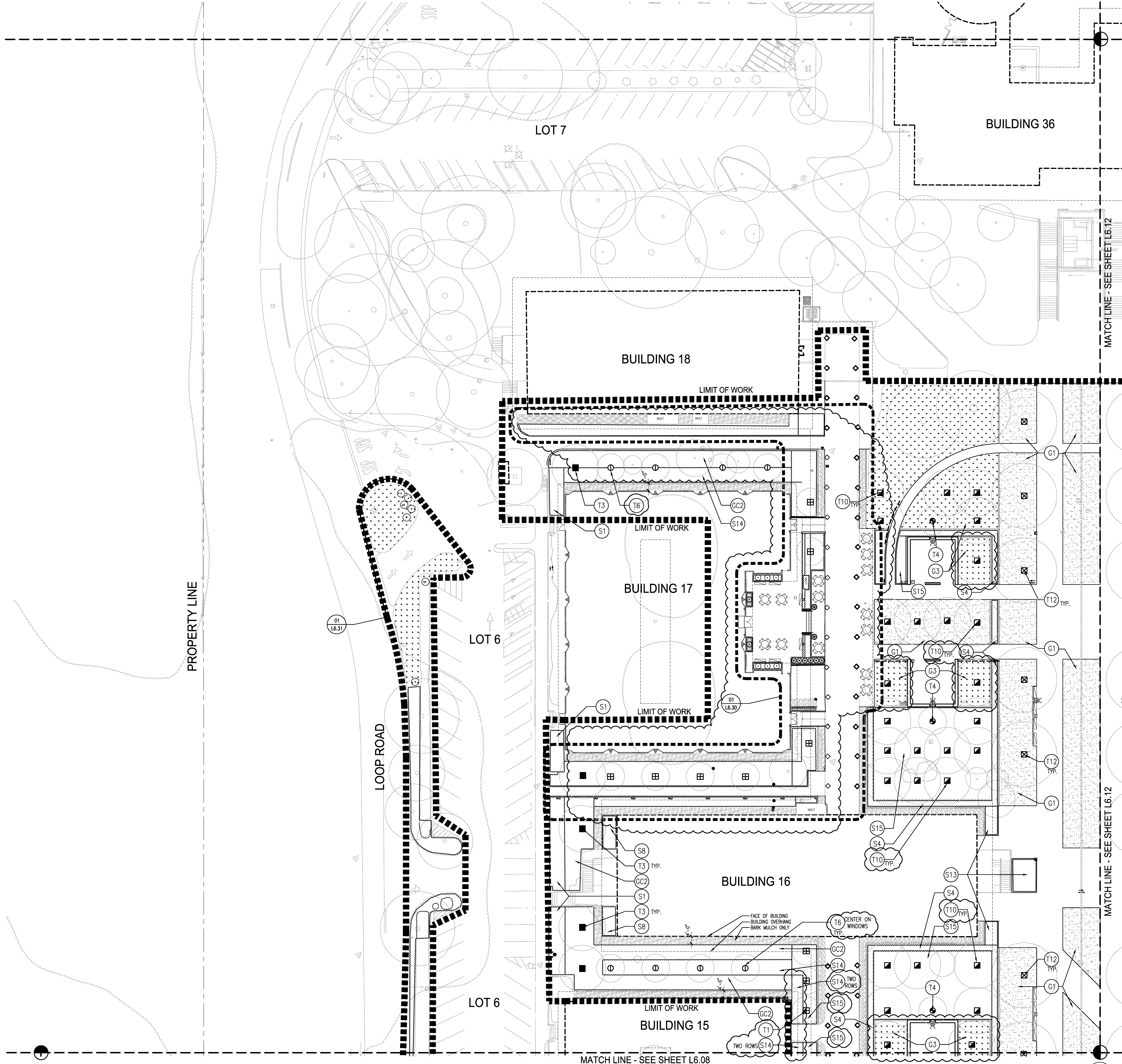
PLANTING PLAN 1" = 20'-0" 01
