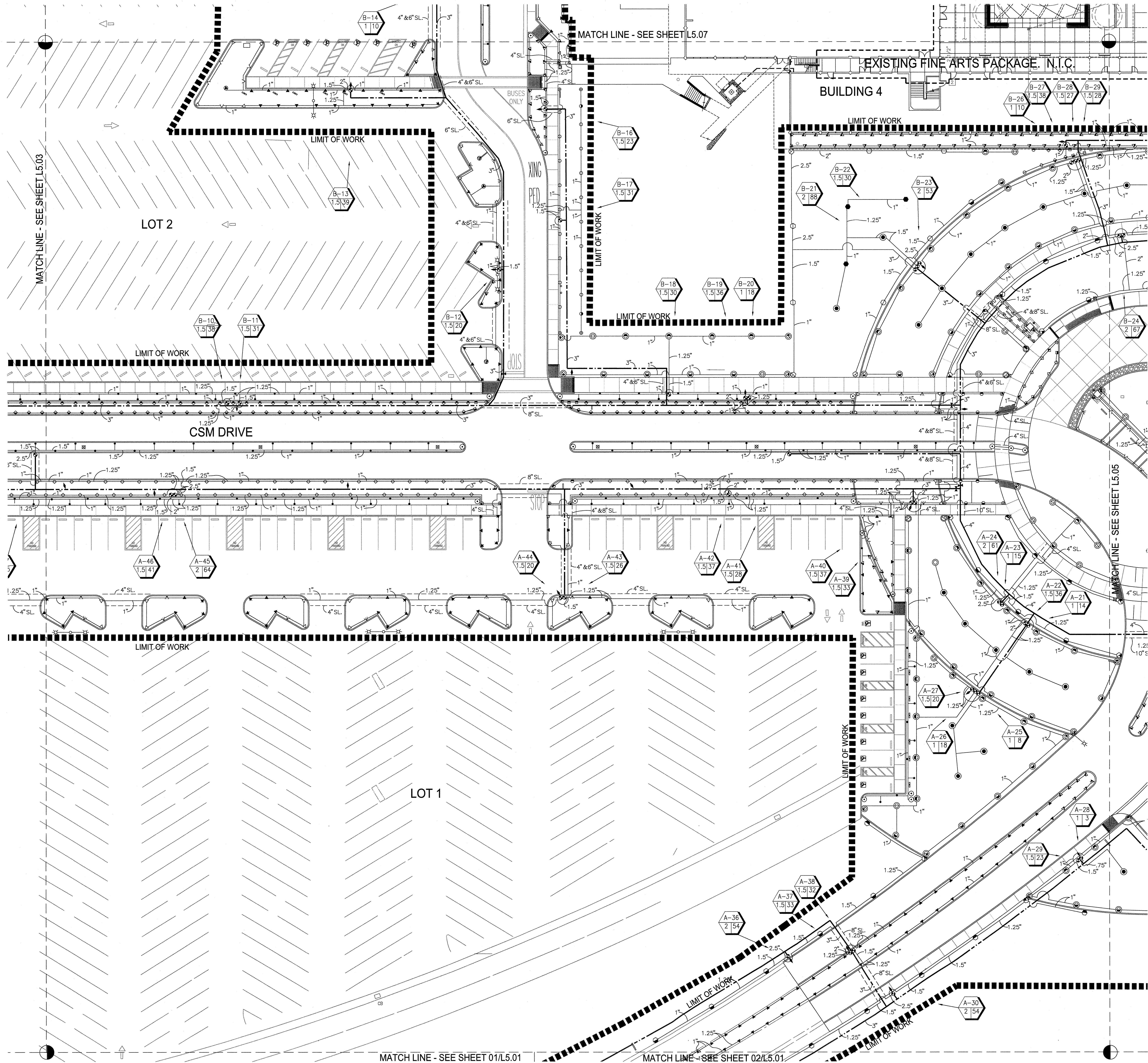
IRRIGATION PLAN 1" = 20'-0"
