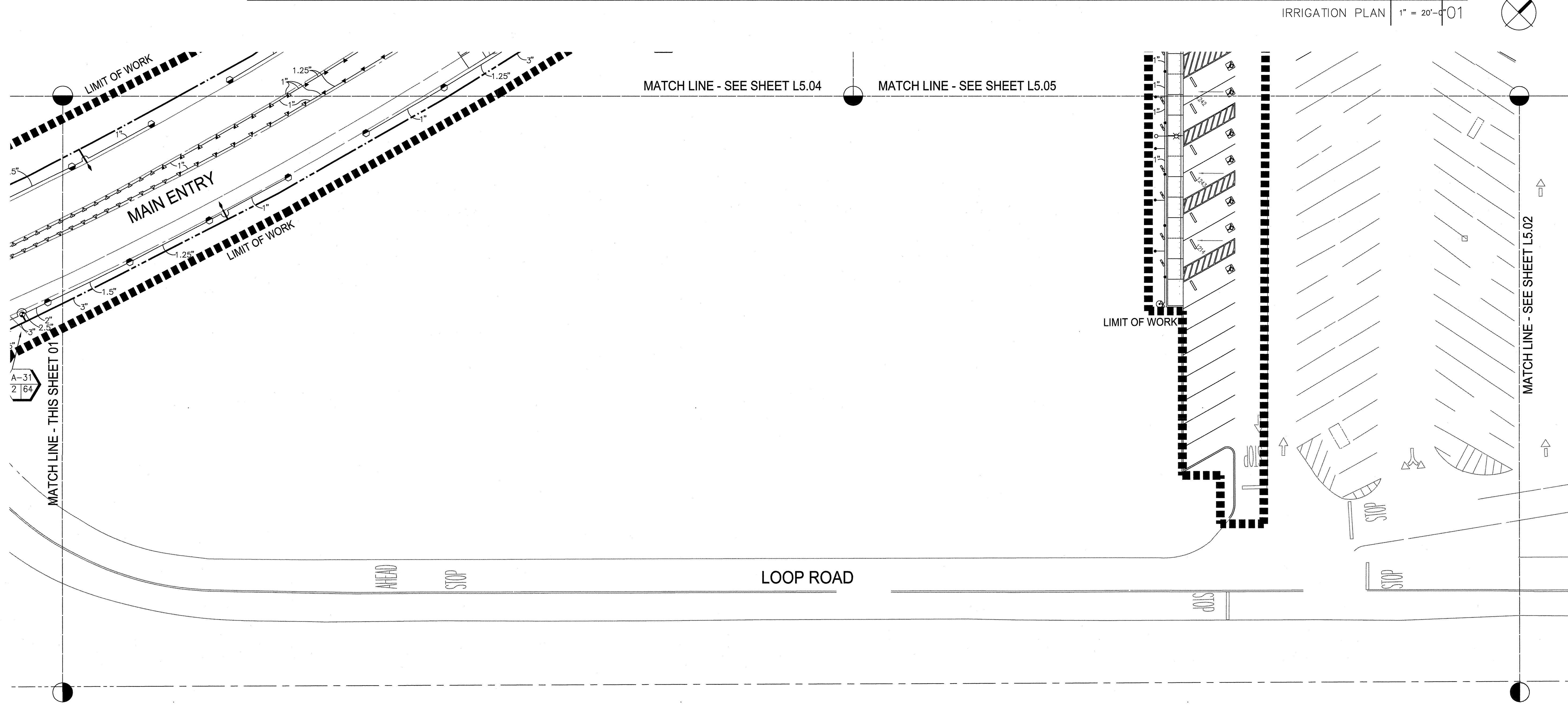
IRRIGATION PLAN | 1" = 20'-0"
