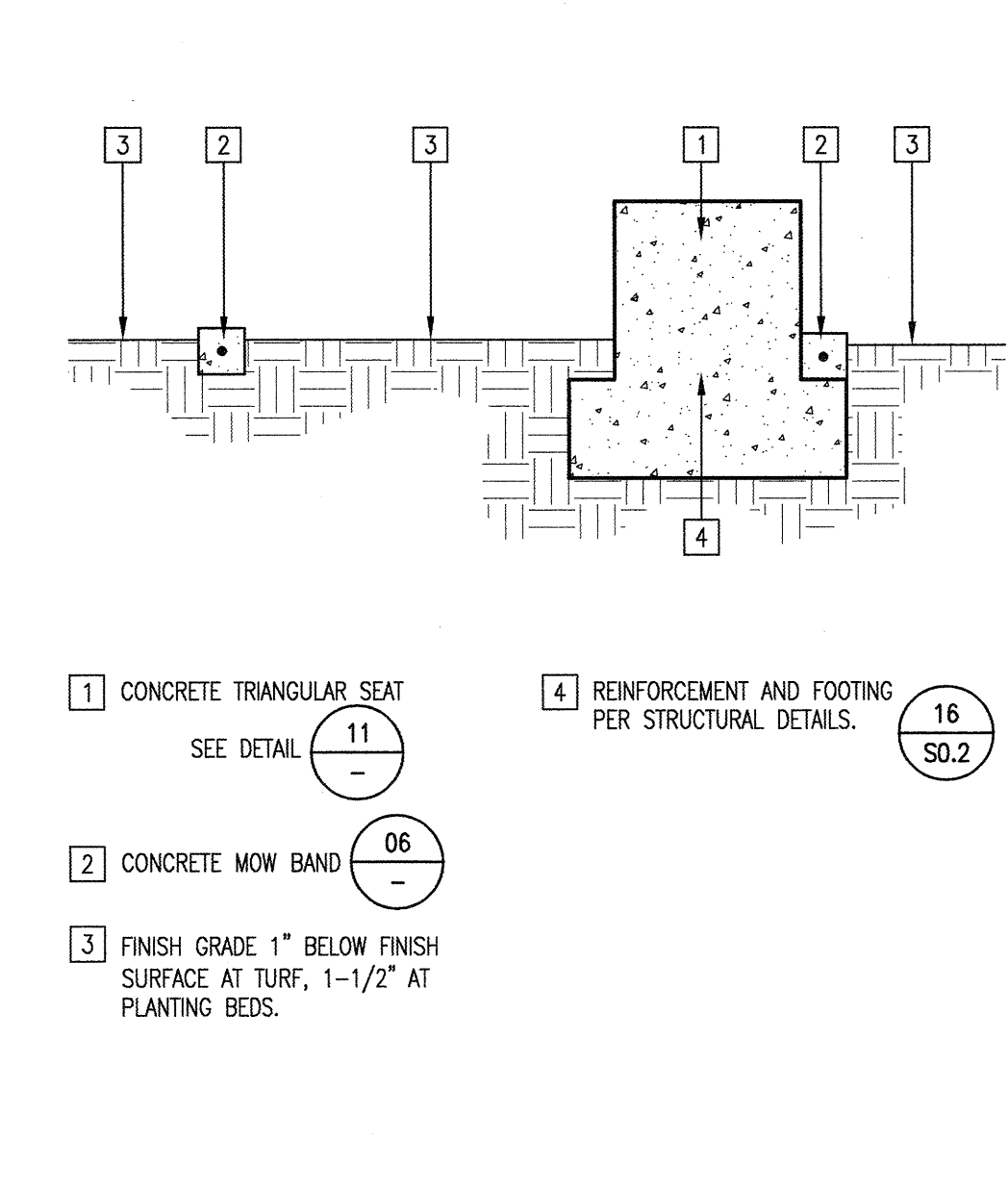
PAVERS AT TRIANGULAR SEAT 1/2" = 1'-0" CSW-TRI2X 12
