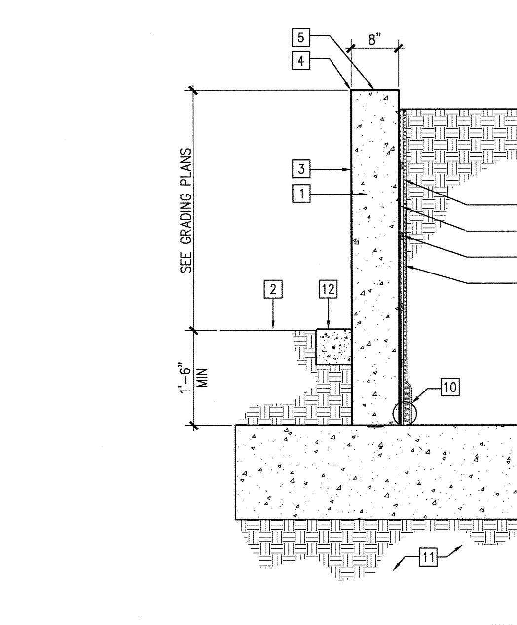
CONCRETE RETAINING WALL TYPE 4 3/4" = 1'-0" CRW-T4 14
