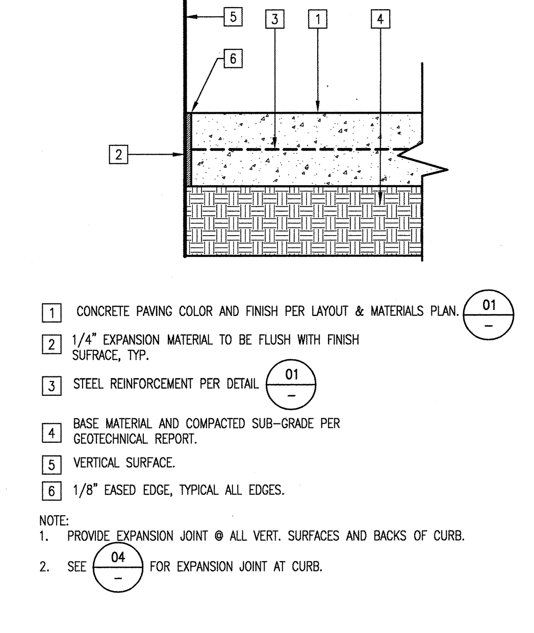
E.J. AT VERTICAL SURFACE 3" = 1'-0" DT02PV35X 07
