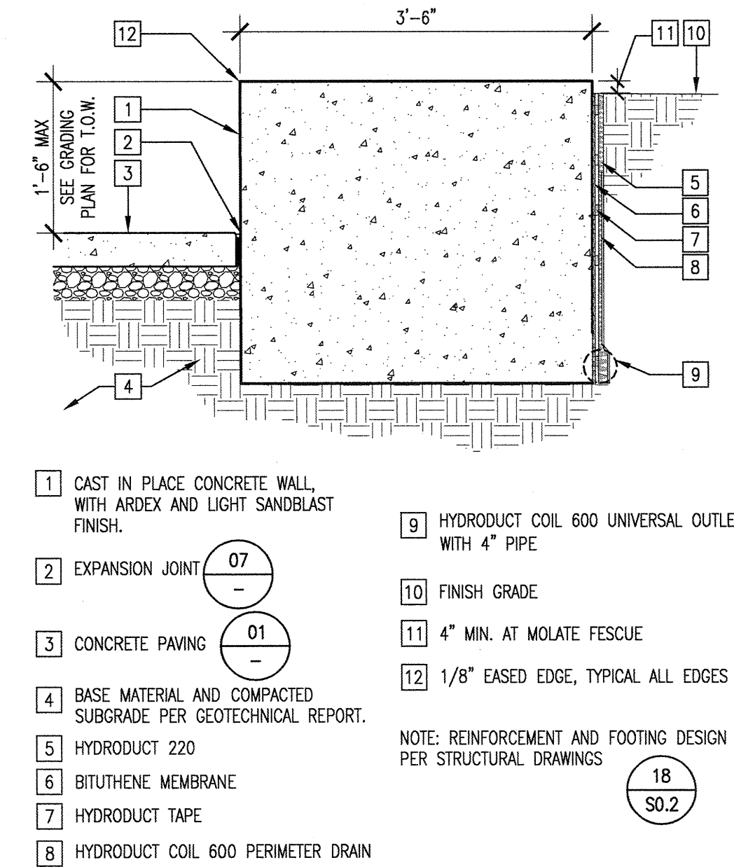
CONCRETE RETAINING WALL TYPE 8 3/4" = 1'-0" CRW-T8 20
