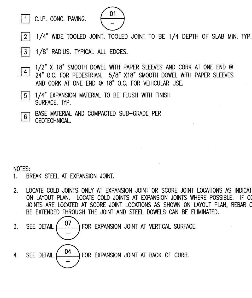
TOOLED CONTROL JOINTS 3" = 1'-0" DT02PV1X2 03
