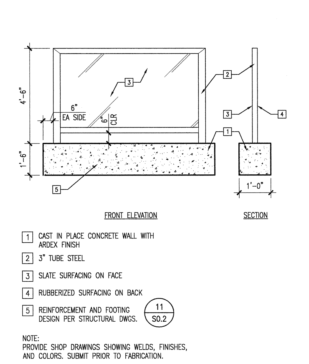
TEACHING STATION BOARD 3/8" = 1'-0" Teaching Station 24
