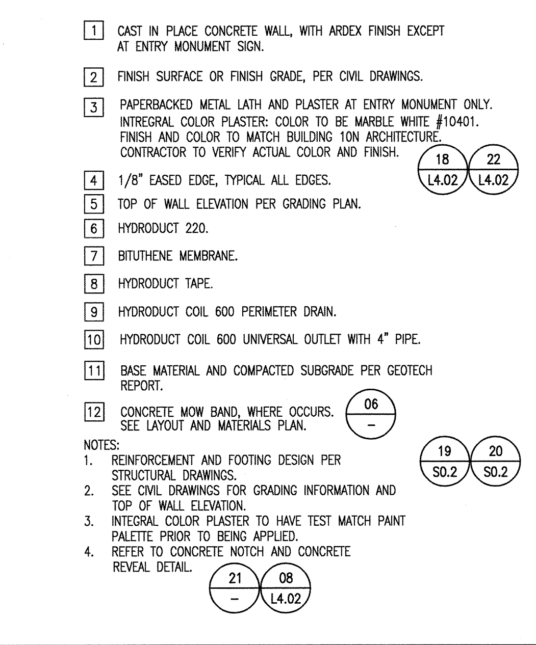
CONCRETE SEATWALL TYPE 2 1" = 1'-0" CSW-T2 10
