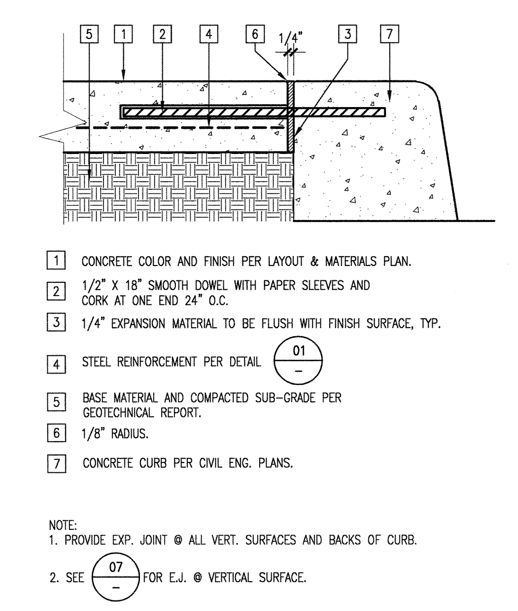
EXPANSION JOINT AT CURB 3" = 1'-0" DT02PV40X 04
