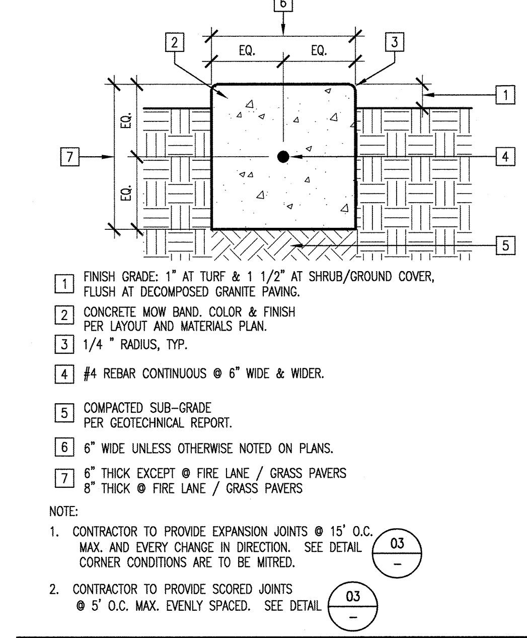
CONCRETE MOW BAND 3" = 1'-0" DT02PV65 06
