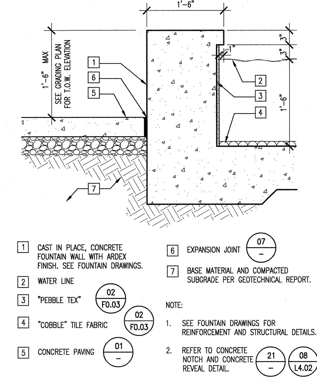
CONCRETE SEATWALL AT FOUNTAIN 1" = 1'-0" CSW-FNTN 13
