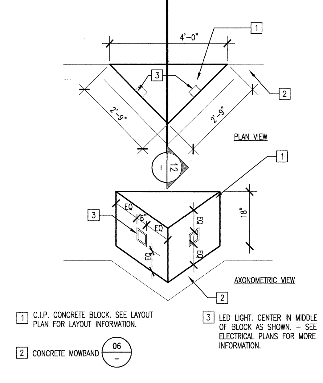
CONCRETE TRIANGULAR SEAT 1/2" = 1'-0" CSW-TRI 11
