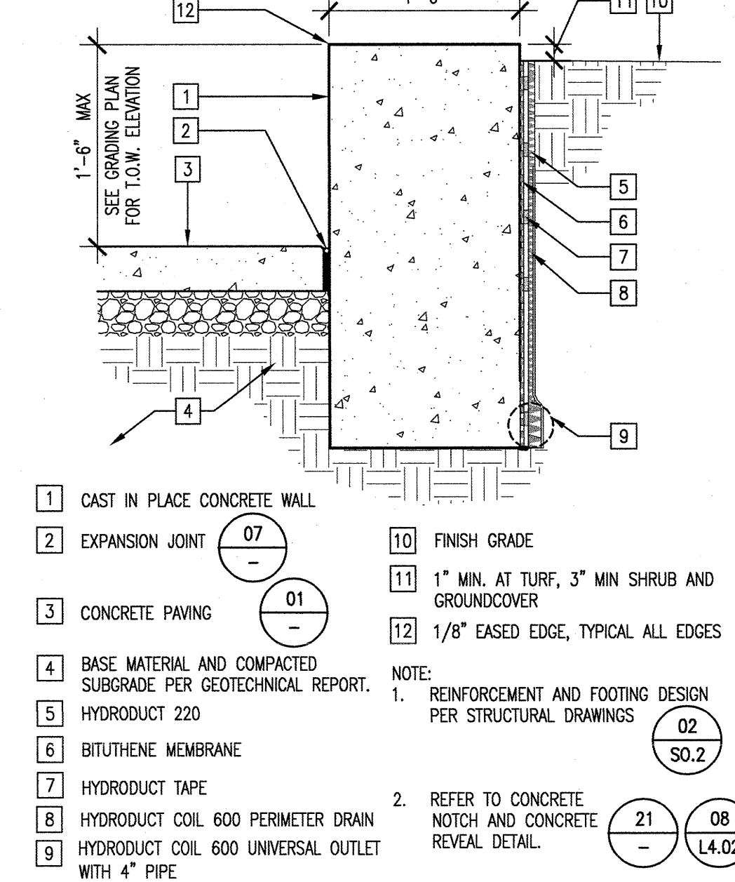
CONCRETE SEATWALL TYPE 4 1" = 1'-0" CSW-T4 09
