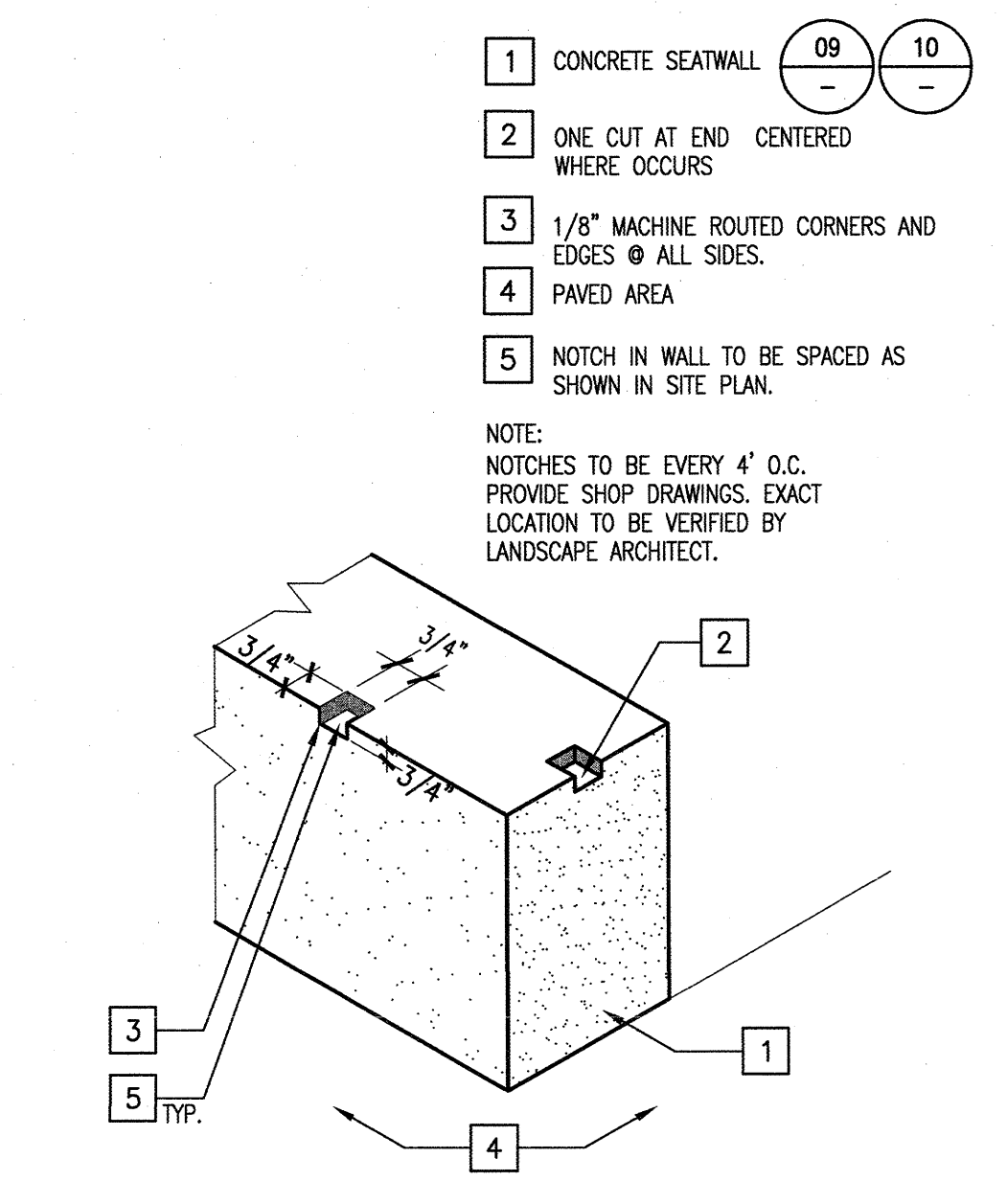
CONCRETE NOTCH 1" = 1'-0" DT02WDS1X 21
