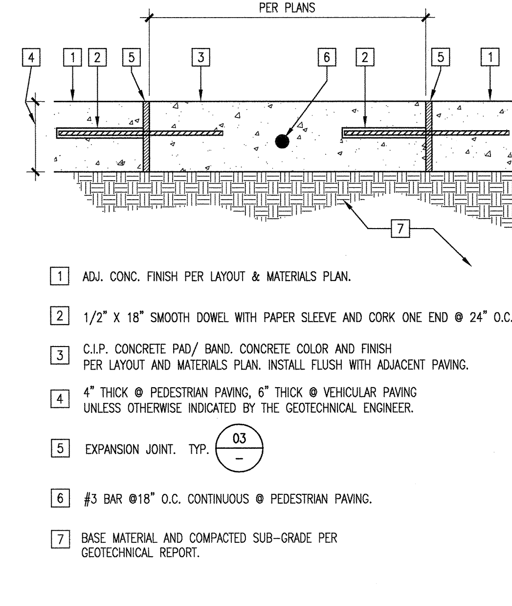
CONCRETE BAND 3" = 1'-0" DT02PV64 08
