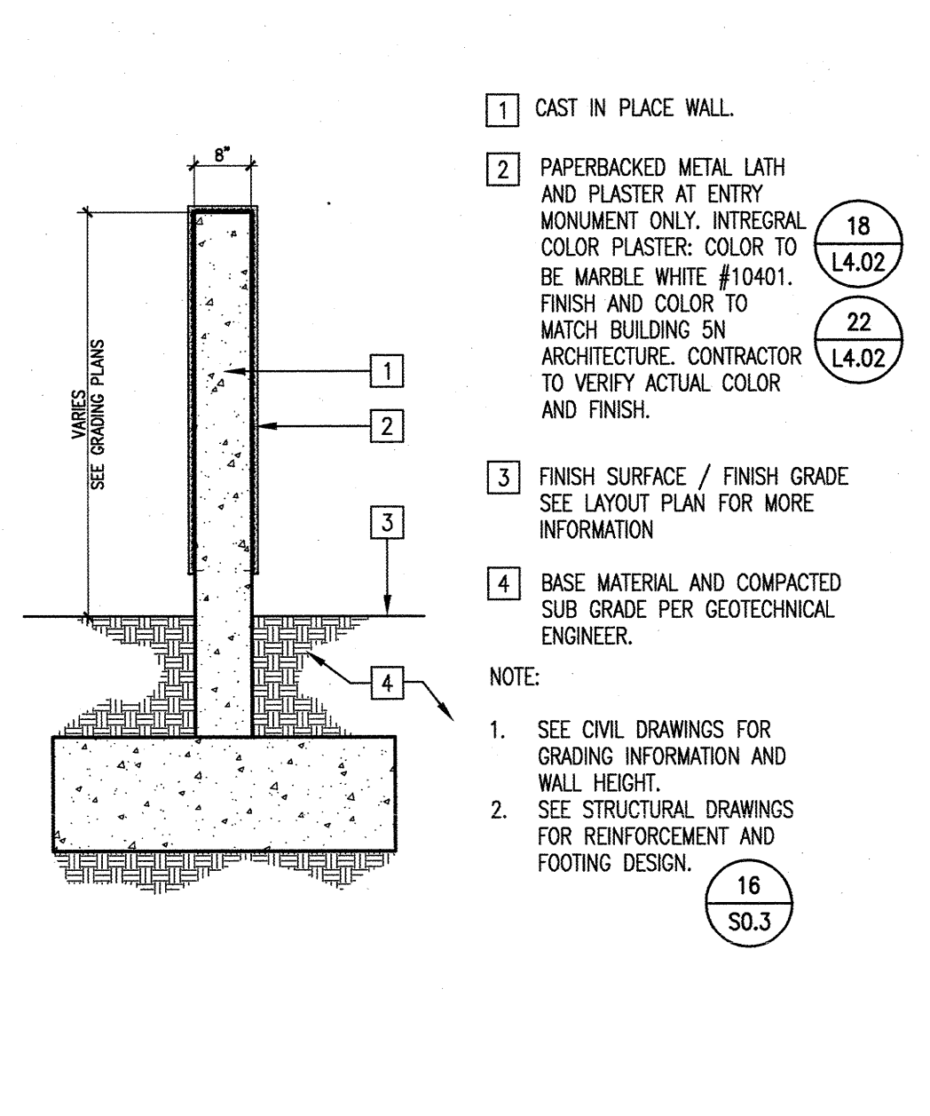
FREESTANDING WALL 1/2" = 1'-0" DT02WD15X 17
