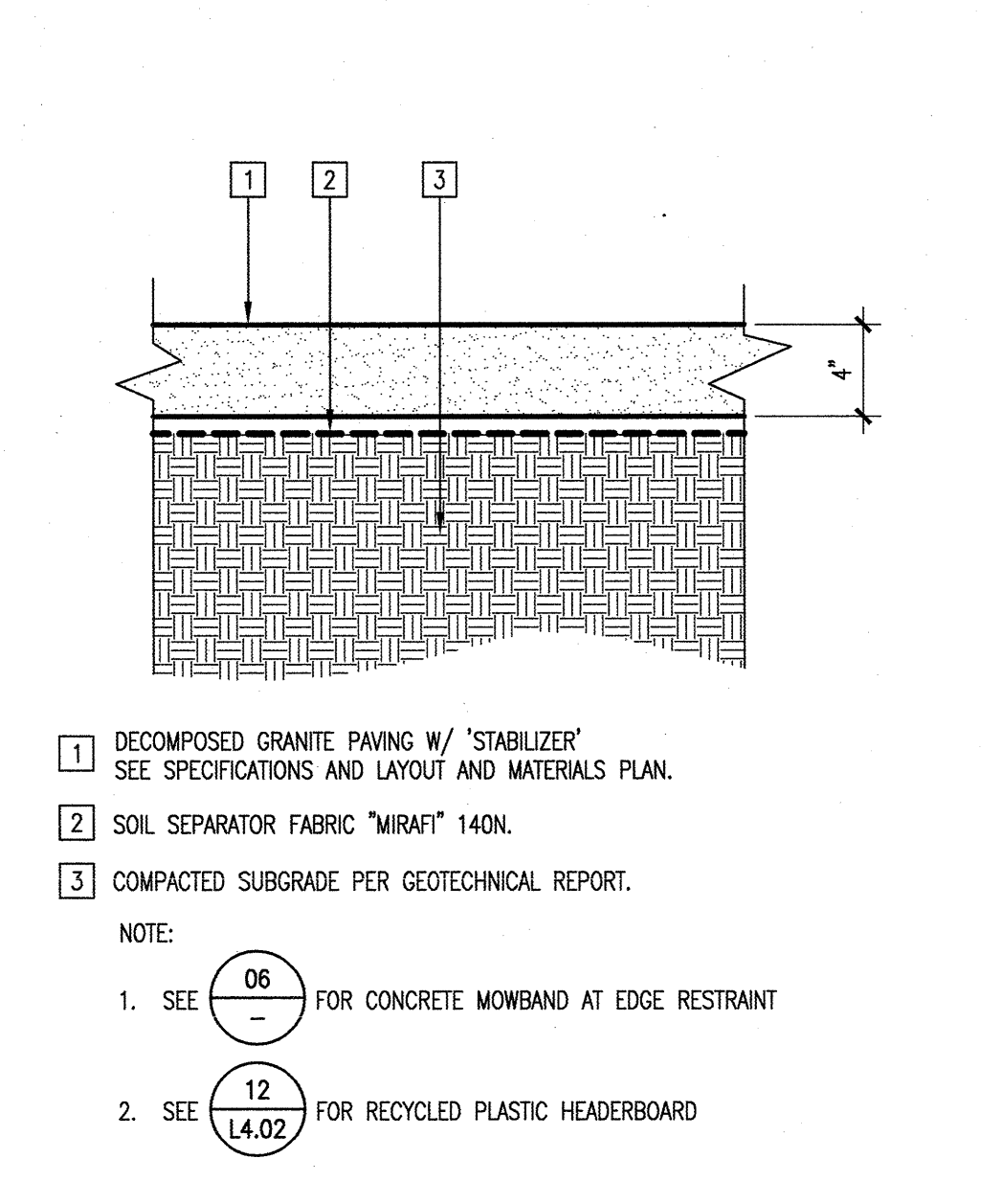
DECOMPOSED GRANITE PAVING 3" = 1'-0" DT02PV16 05
