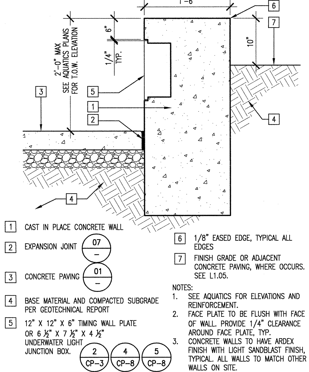
AQUATICS UTILITY WALL 1" = 1'-0" CSW-T5 22
