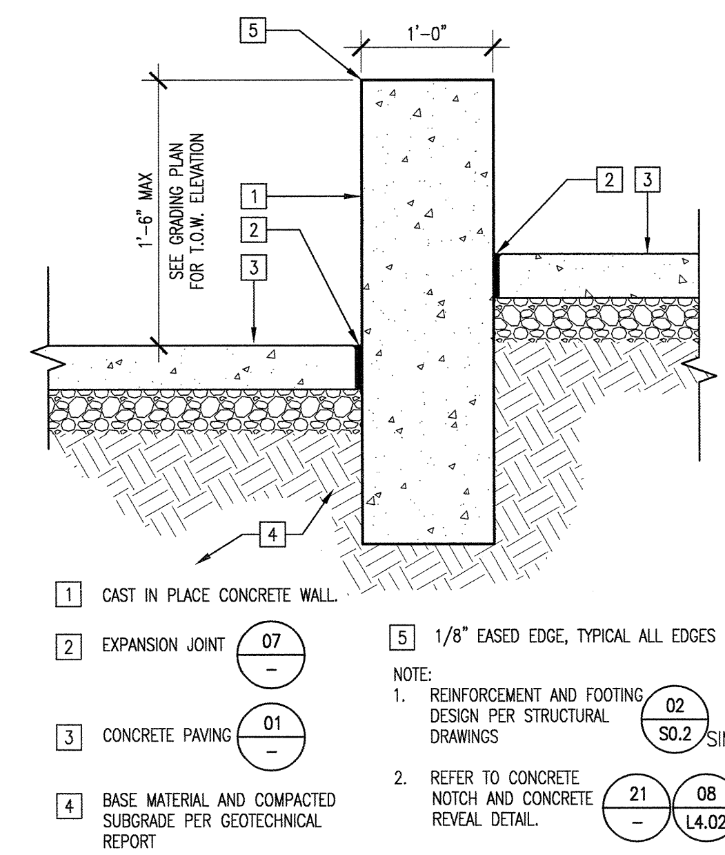
CONCRETE SEATWALL TYPE 3 1" = 1'-0" CSW-T6 16
