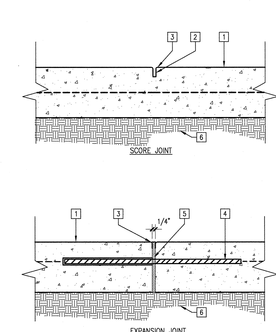
CONCRETE PAVING 3" = 1'-0" DT02PV10 01
