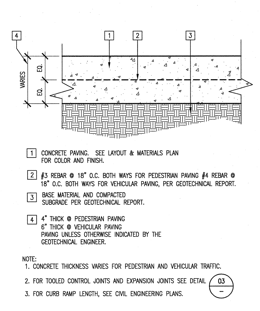
CONCRETE PAVING 3" = 1'-0" DT02PV10 01
