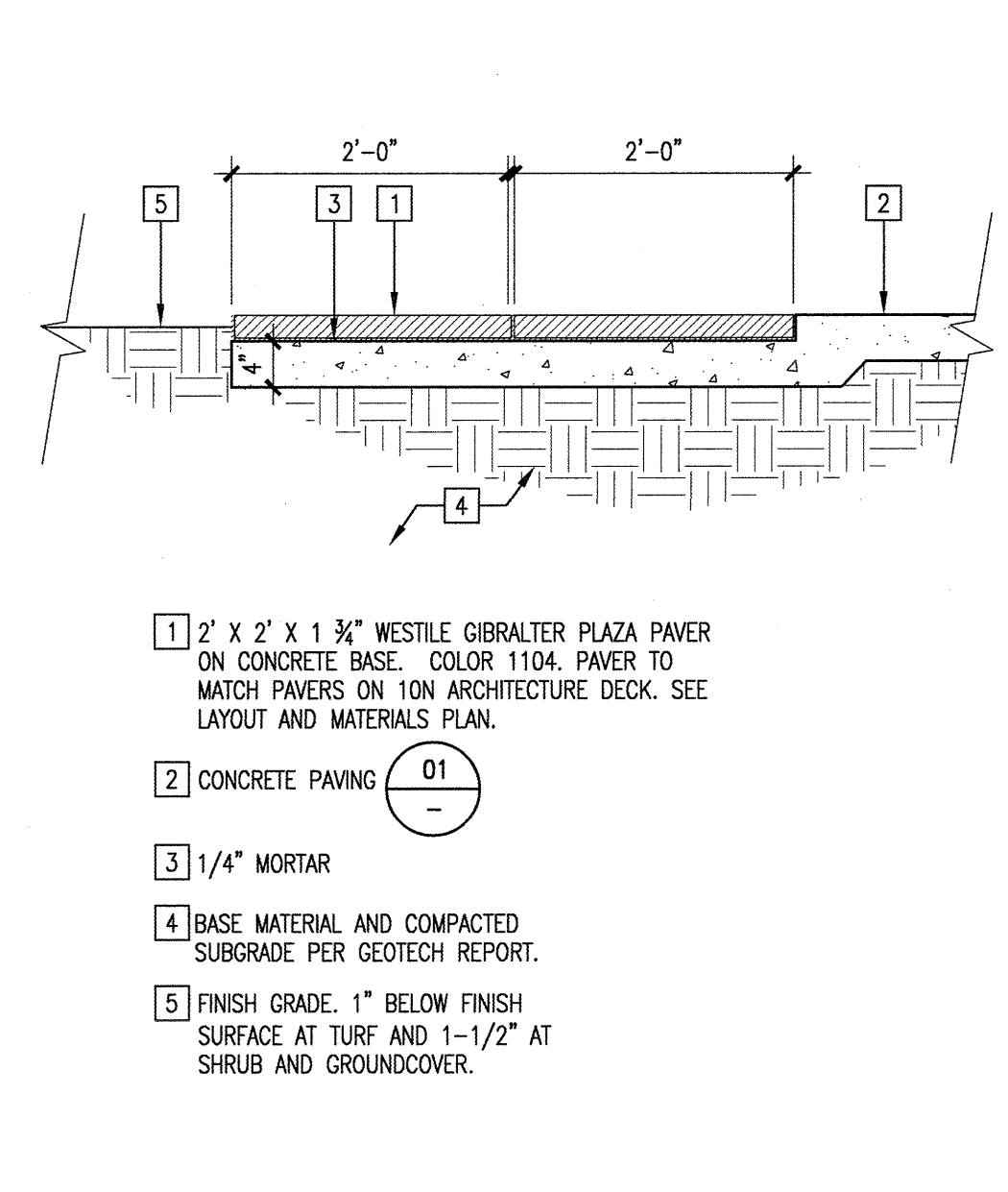
PAVERS 3/8" = 1'-0" DT02PV68 23
