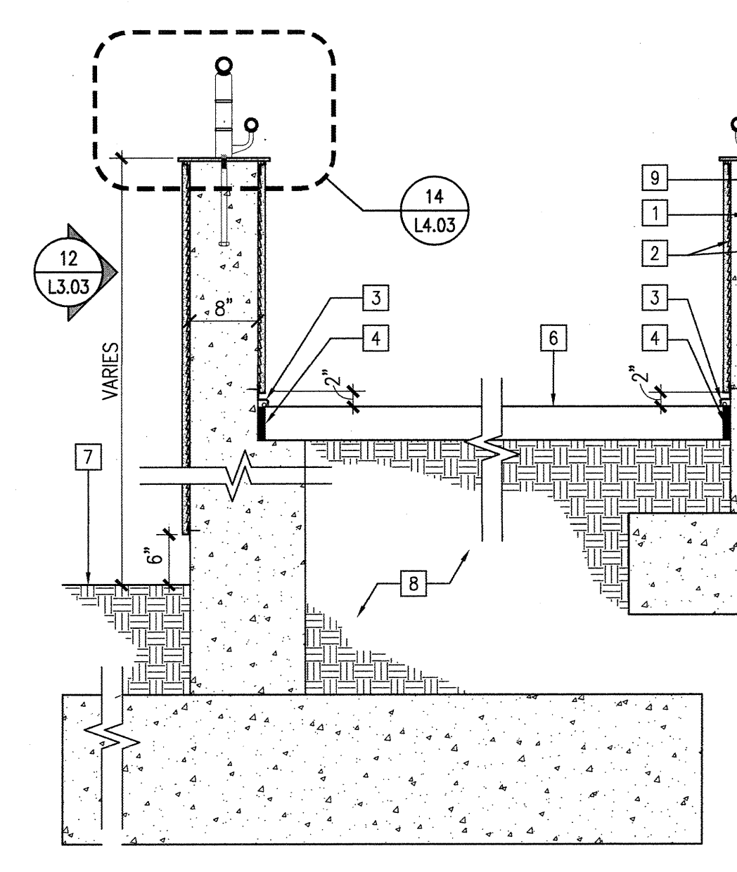
SECTION AT 10N STAIRS 3/4" = 1'-0" CRW-T2 15
