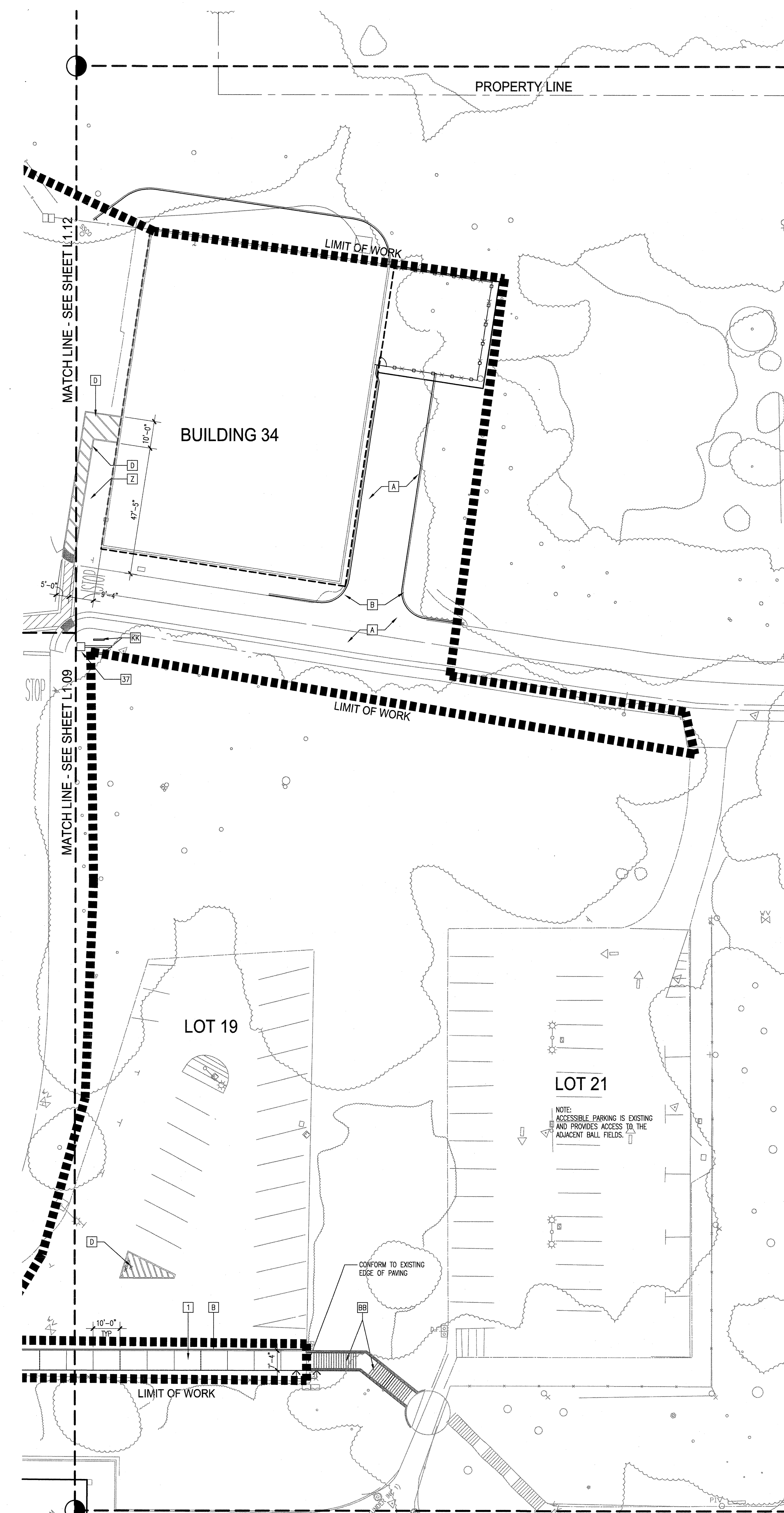
LAYOUT AND MATERIALS PLAN 1" = 20'-0" 01
