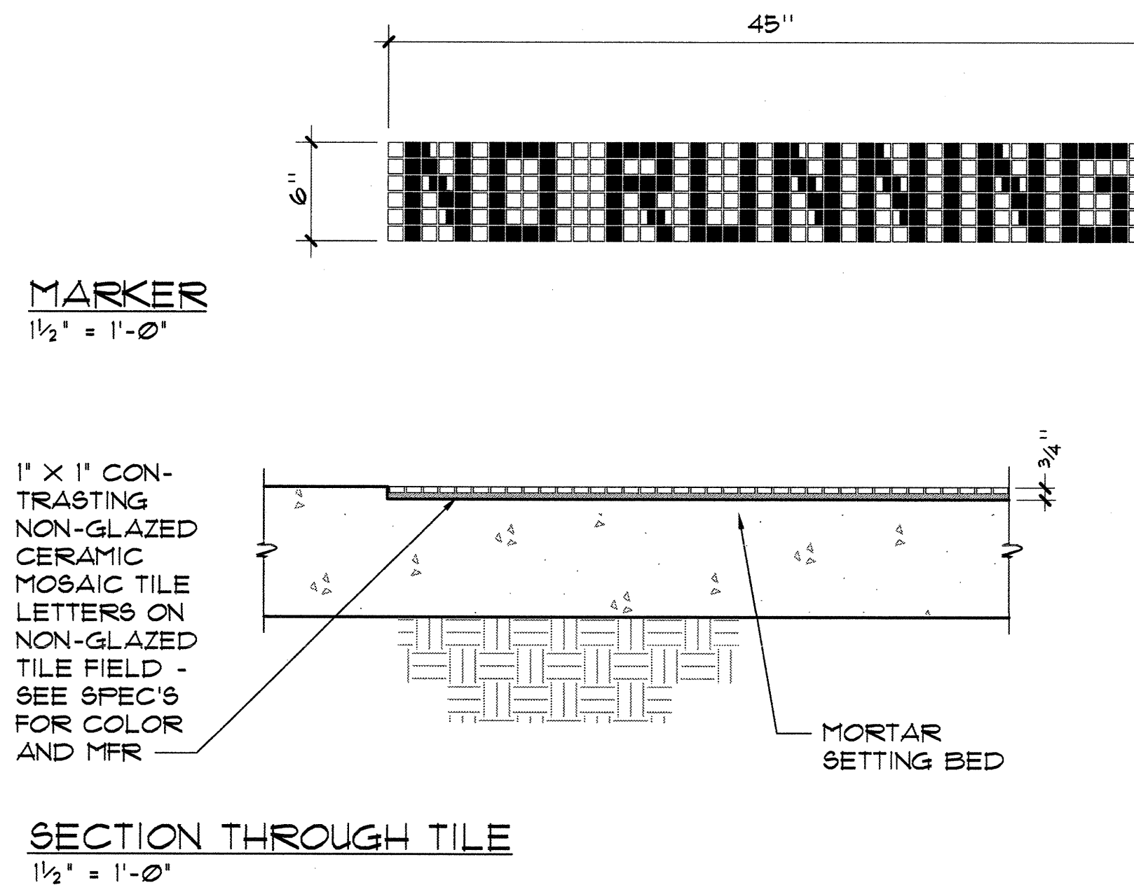
2 SECTION THROUGH TILE 1/2" = 1'-0"
