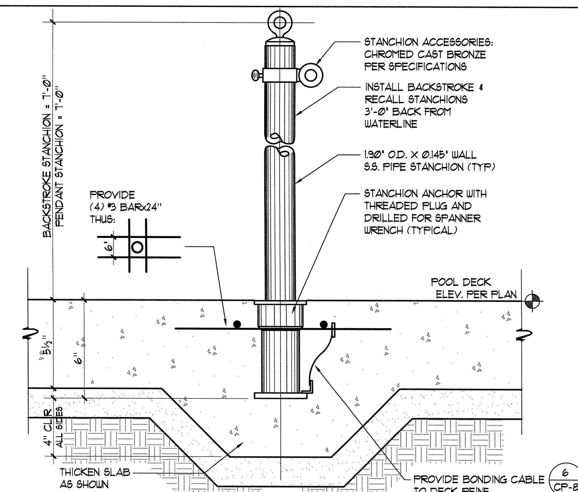
8 STANCHION POST/ANCHOR 3/4" = 1'-0"
