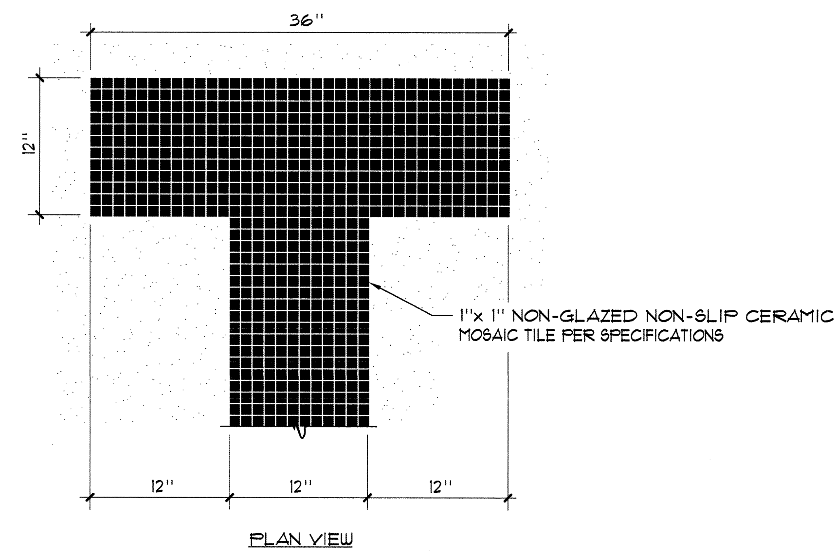
1 RACING LANE LINE 1/2" = 1'-0"
