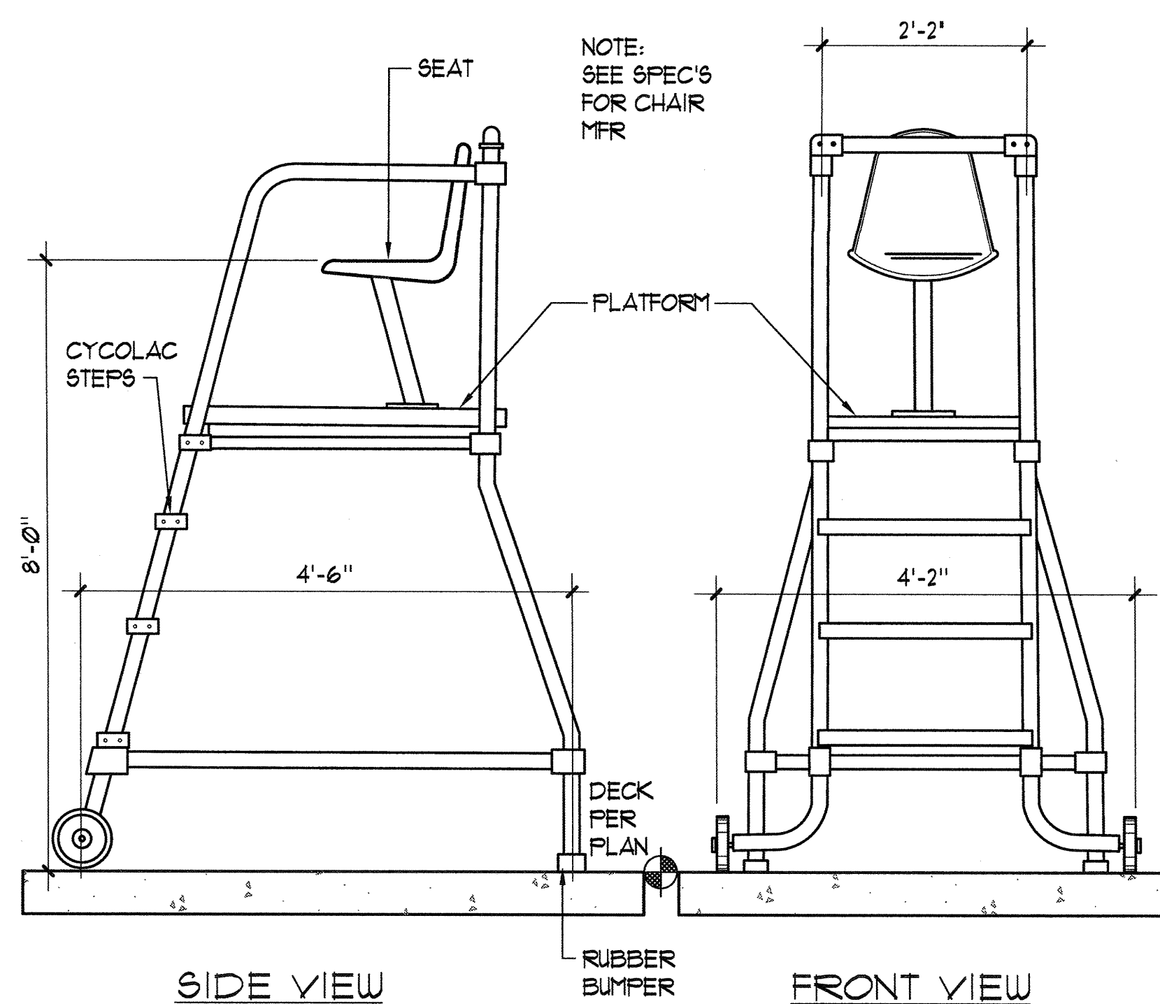
6 MOVEABLE LIFEGUARD CHAIR NO SCALE
