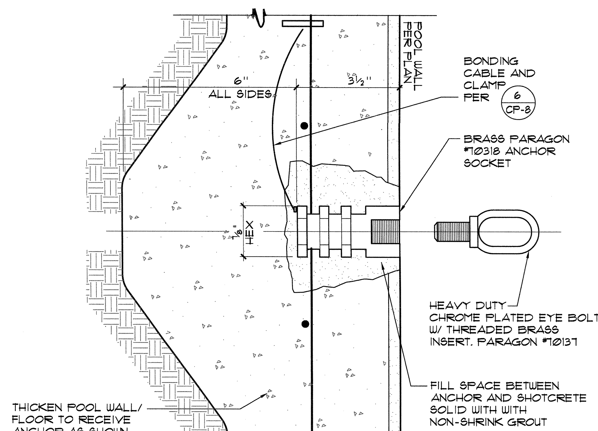
5 DISABLED LIFT 3/4" = 1'-0"
