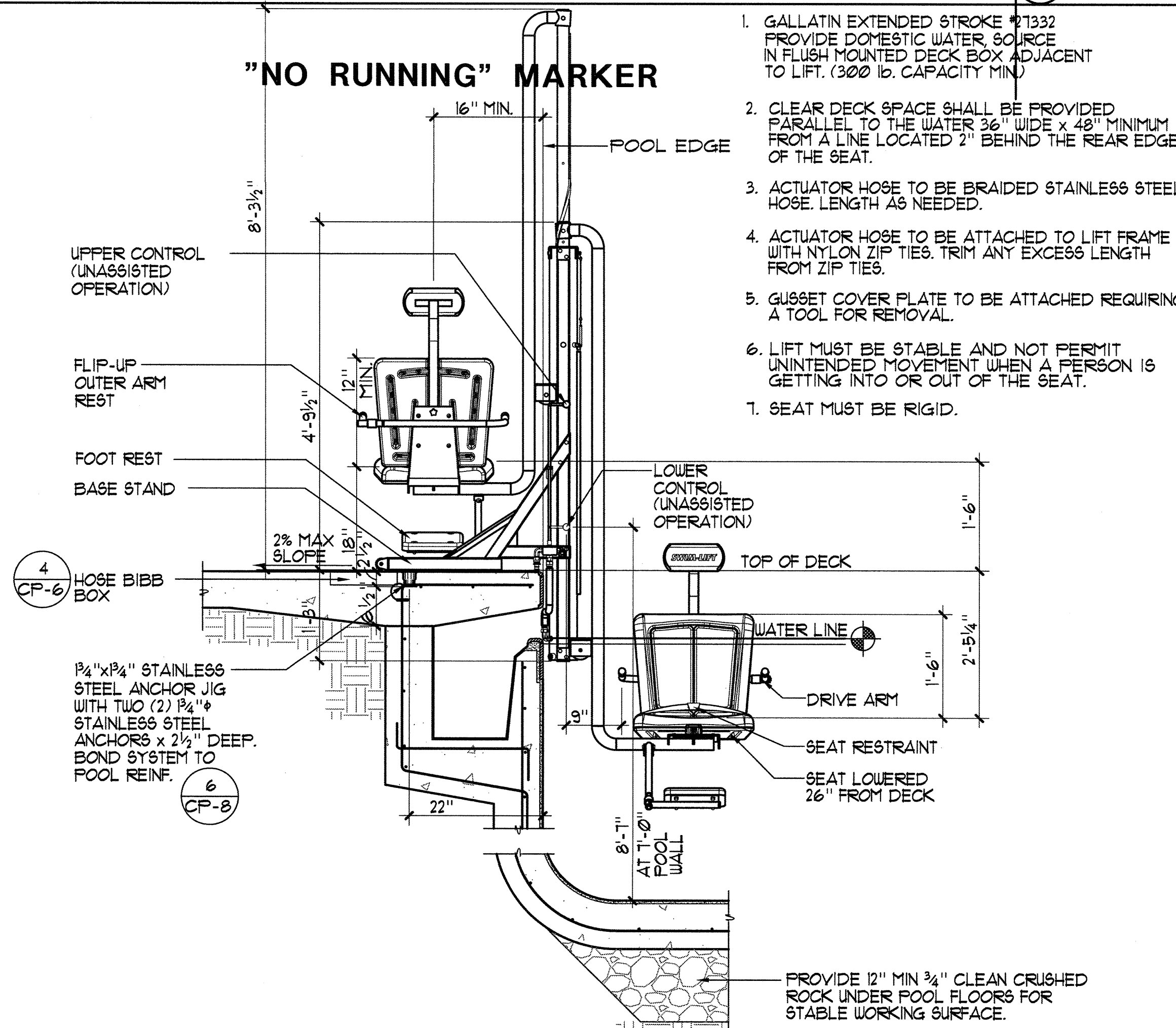
5 DISABLED LIFT 3/4" = 1'-0"
